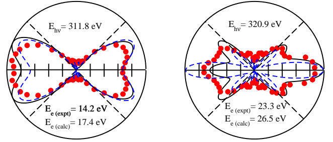
FIG. 8: (Color online) Photoelectron angular distributions for \text{C}(1s^{-1}) ionization, photon polarization parallel to molecular axis. Solid curves: fixed-nuclei cross sections averaged over asymmetric-stretch and bending modes; broken curves: fixed-nuclei cross sections at equilibrium geometry. E_{e(\text{expt})} and E_{e(\text{calc})} refer to the experimental photoelectron energy and the energy used in the calculation, respectively (see text). Experimental points from Liu et al. [3]
