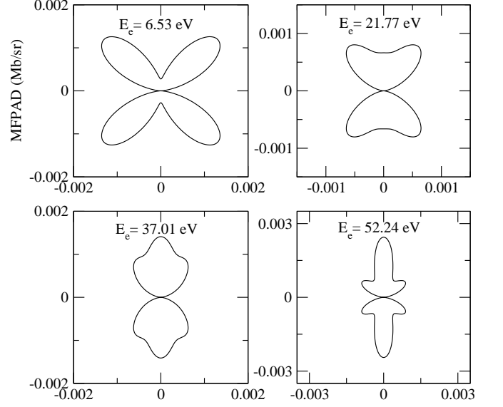
FIG. 6: As in Fig. 4, for perpendicular polarization. Calculations done using ion orbitals.
