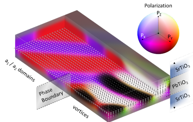
Figure 1. Colorized phase field model of the a-domain / vortex boundary for one of the PbTiO 3 layers within a PbTiO 3 (16u.c.)/SrTiO 3 (16u.c.) superlattice. A net axial polarization is predicted for the vortex region matching the sign of the P Y component of the neighboring a 1 /a 2 domains.
