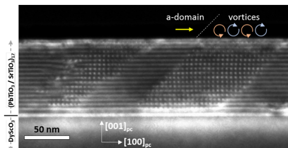
Figure 2. Dark field TEM image showing ferroelectric vortices and a-domain coexistence in a PbTiO 3 (8u.c.) / SrTiO 3 (8u.c.) superlattice. Image formed from the [00\bar{4}]_{pc} reflection.
