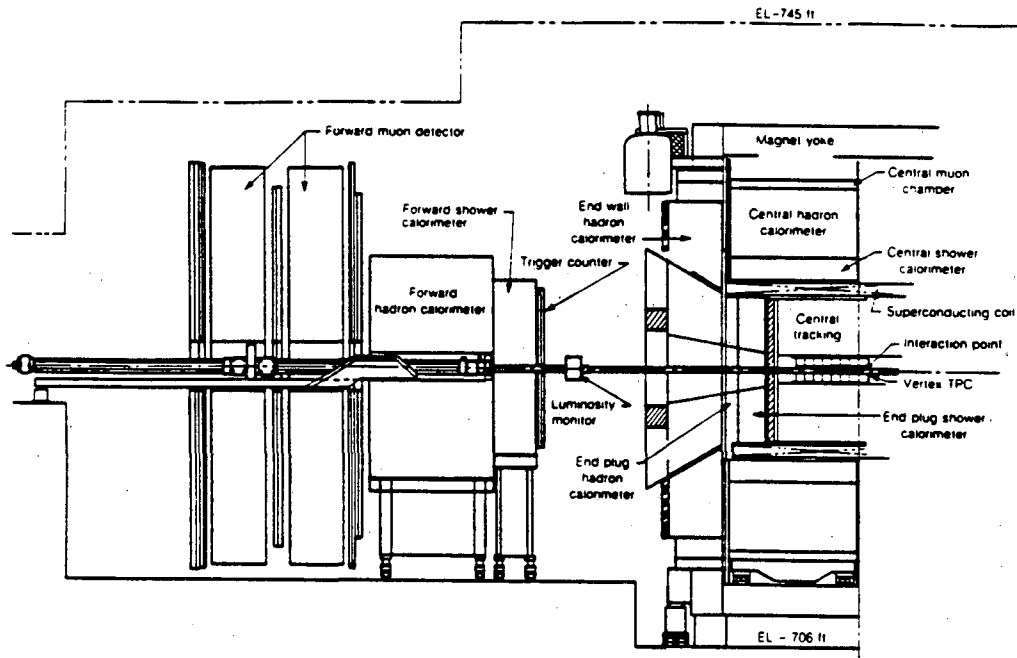
Fig. 3. Side view of the CDF Detector 7] .
