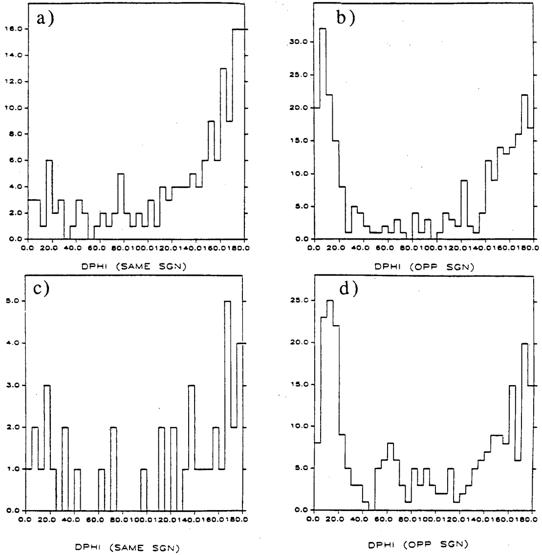
Fig. 10. The azimuthal opening angle for the same sign e\mu samples in a) the e\mu trigger data ( 1.8pb^{-1} ) and c) the b\bar{b} Monte Carlo, and for the opposite sign e\mu sample in b) the data and d) the b\bar{b} Monte Carlo.
