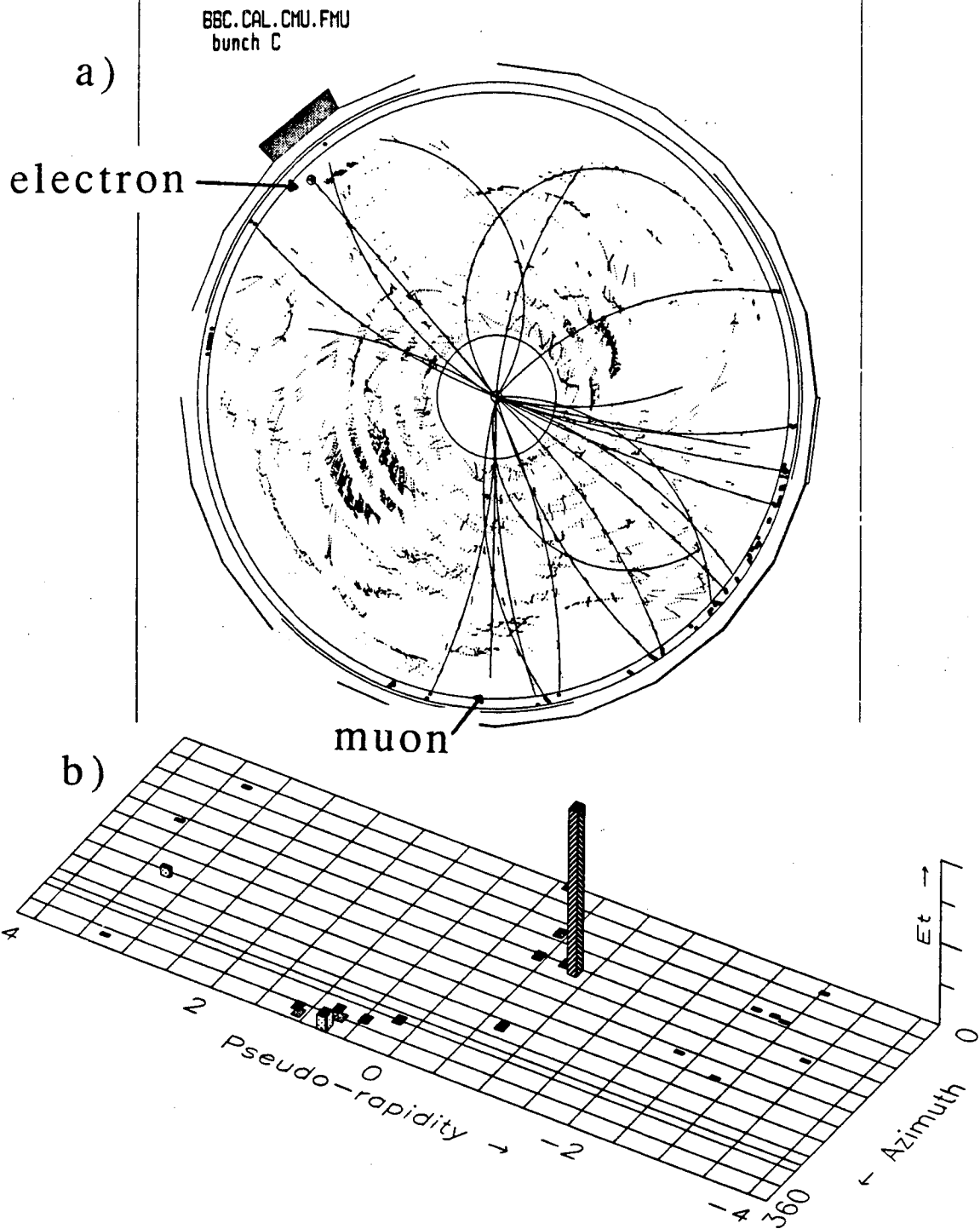
Fig. 12. The one candidate event. a) the r\phi view: the electron at \phi=130^\circ has E_T=31.7 GeV, the \mu at \phi=260^\circ has P_T=42.5 GeV/c. b) the azimuth vs. \eta plot, with the vertical scale representing the calorimeter energy. The electron is the large tower at \phi=130^\circ , the \mu is at \eta=-0.7 and \phi=260^\circ .
