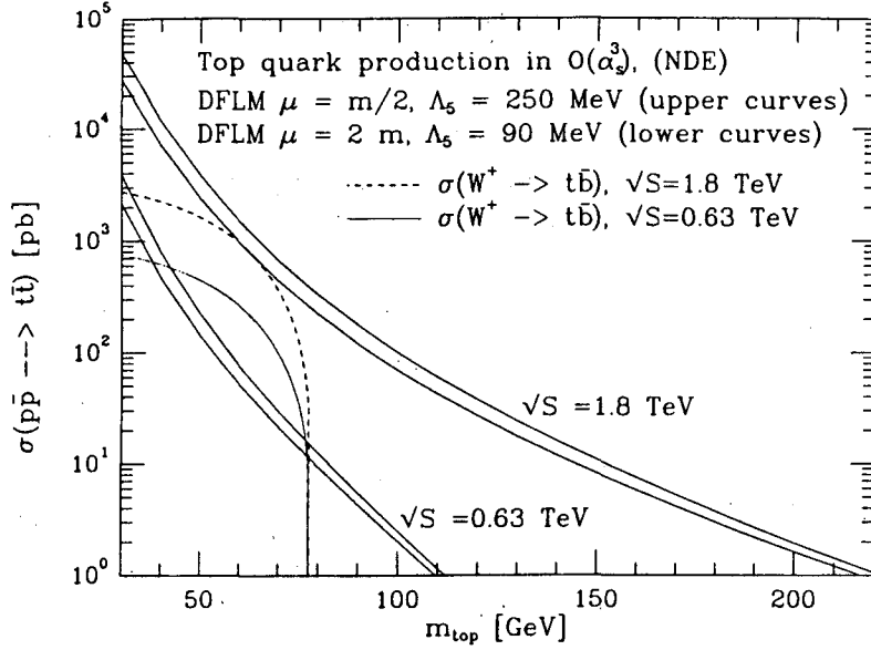
Fig. 1. Top pair production cross section versus top mass, as calculated by K. Ellis 8] , using the method of Altarelli et al. 11] . The next to leading order calculations of Nason et al. 9] and the DFLM structure functions 10] are used. The bands represent the uncertainty due to \mu scale and the range in \Lambda_5 . The W \rightarrow t\bar{b} cross section is also included.
