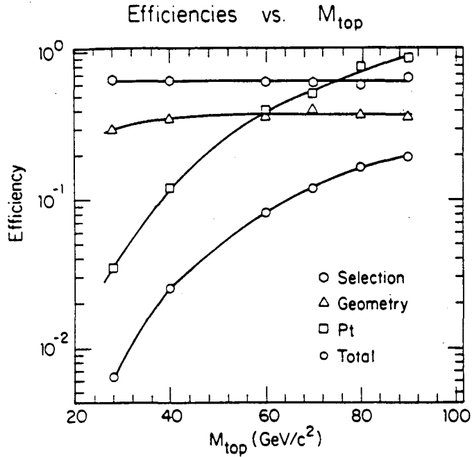
Fig. 13. Detection efficiencies for e\mu pairs from t\bar{t} production, as a function of the top mass, for: i) the P_T requirement; ii) the geometric acceptance (both \eta and fiducial cuts); iii) the dilepton identification cuts, and iv) total. The branching ratio into e\mu is assumed to be 100% in this plot.
