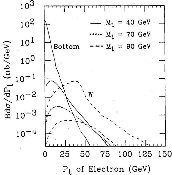
Fig. 2. Inclusive P_{\perp} distribution of the electron from top and bottom semileptonic decays and for W \rightarrow e\nu , calculated using the PAPAGENO Monte Carlo 13] . Only the branching ratio into electron has been included in the rate, i.e., no detector simulation is included.
