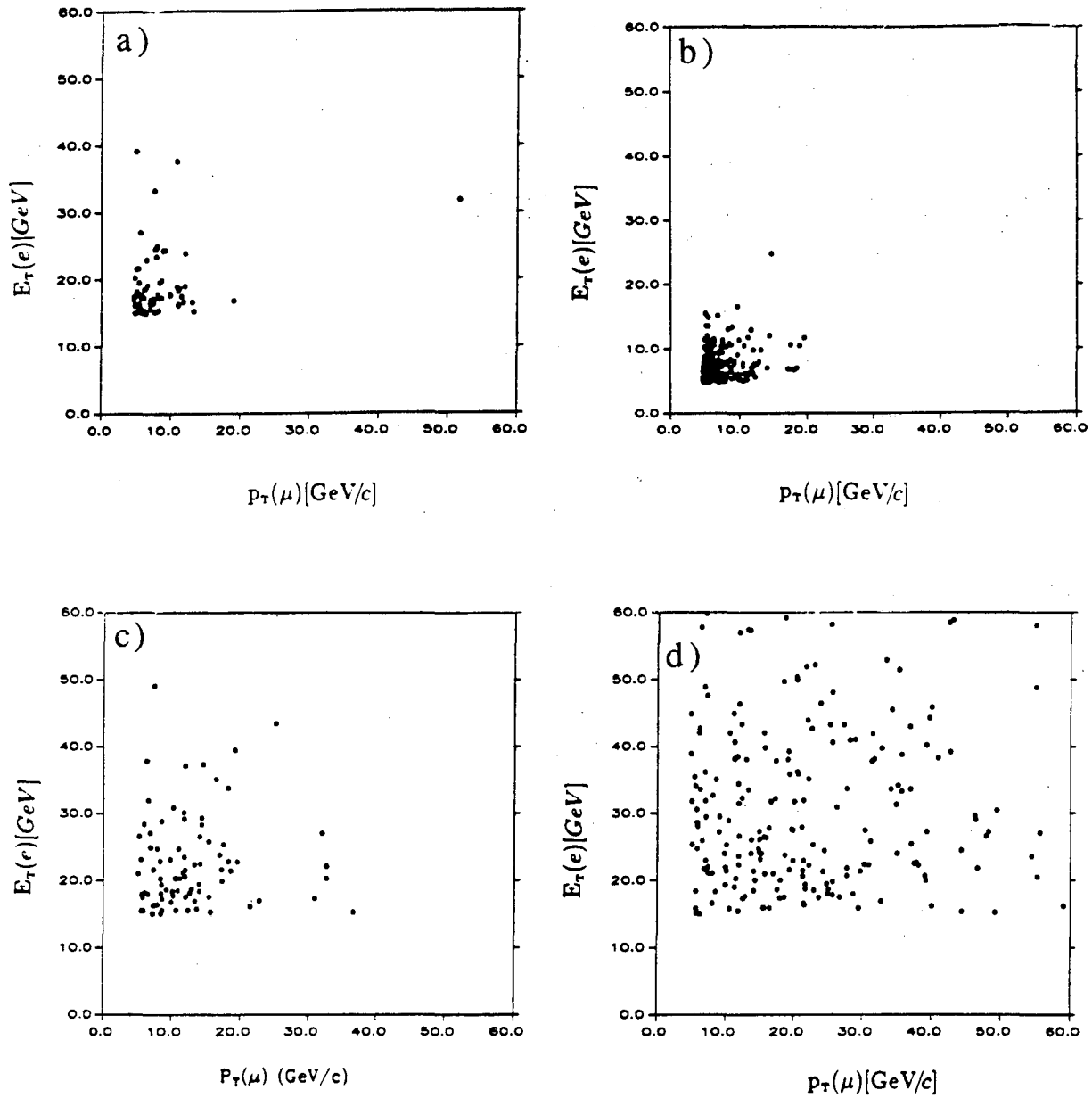
Fig. 7. Scatter plots of the electron E_T versus the muon P_T for a) the data ( 4.4 \text{ pb}^{-1} ); b) the b\bar{b} Monte Carlo ( 0.64 \text{ pb}^{-1} ); and top Monte Carlo c) for M_{top}=28 \text{ GeV} ( 2.1 \text{ pb}^{-1} ), and d) for M_{top}=70 \text{ GeV} ( 79 \text{ pb}^{-1} ).
