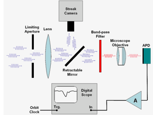
Fig. 1. Schematic diagram of the experimental set-up used for the measurement at BL 7.2.
