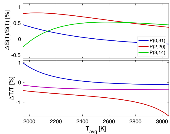
Fig. 20 The relative difference between \overline{S(T)} and S(\bar{T}) for the P(0,31), P(2,20) and P(3,14) (top) and the difference between \bar{T} and the temperature inferred from the \overline{S} for the P(0,31) line (blue), the P(2,20) line (red) and from their ratio (purple)
