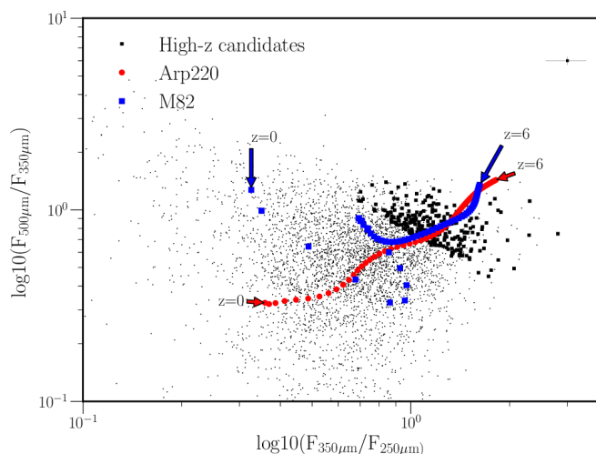
Fig. 2. Colour-colour diagram of the SPIRE fluxes with the tracks of the local starburst galaxies M82 (blue) and Arp220 (red) over-plotted. The tracks represent the observed colours as expected from the same SEDs observed at different redshifts from z = 0 to z = 6 with redshift steps of \Delta z = 0.1 . The bold points are the high- z candidates which lie in the same colour space than the evolved tracks at z > 2 . The upper right area of the plot shows the average error bar for the high- z candidates. All these methods are based on MBB models, where the redshift evolution of the SEDs is not included. Therefore, more sophisticated SED templates should be used to investigate the correlation between redshift and colours.
