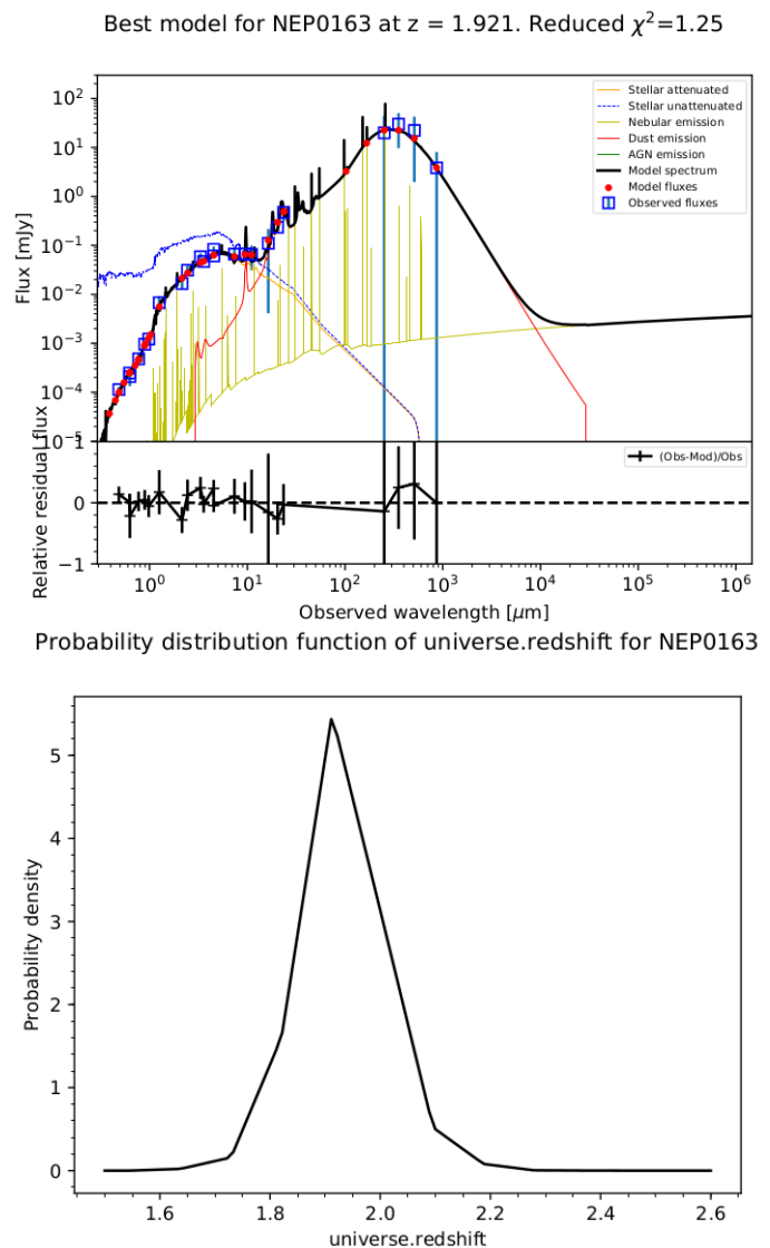
Fig. 4. (Left panel) Example galaxy SED fit from our sample produced by CIGALE with the modules taken into account in the legend. The blue squares are the observed fluxes in mJy, the red dots represent the corresponding predicted fluxes by CIGALE that lie on the black line model fit. Bruzual & Charlot (2003) reproduces the stellar component, where the orange line is the stellar attenuation whereas the blue line shows the unattenuated stellar emission. The green line is the AGN component, modelled by the Fritz et al. (2006) (no green line implies no AGN presence). The dust component is represented by the red line (Draine et al. 2014). The emission lines are shown in pale yellow. The upper part of the plot shows the ID of the source, the redshift and the reduced \chi^2 fit result. (Right panel) Corresponding probability distribution function (PDF) of the estimated photometric redshift for the source in the left panel. The PDF peaks at redshift z_{\text{phot}} = 1.9 . CIGALE produces a Bayesian analysis for each parameter selecting the most likely result.
