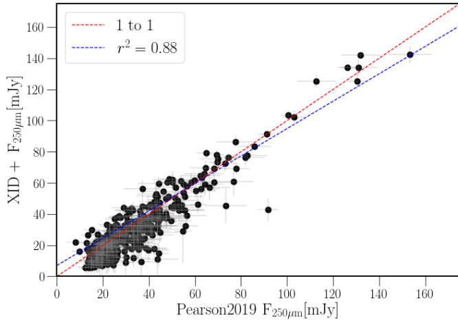
Fig. A.1. Comparison of the SPIRE 250 \mu\text{m} band fluxes from the catalogues of Pearson et al. in prep (x-axis) and HELP (y-axis), finding a good agreement between them. Also shown are the 1-to-1 line and r^2 regression line.
