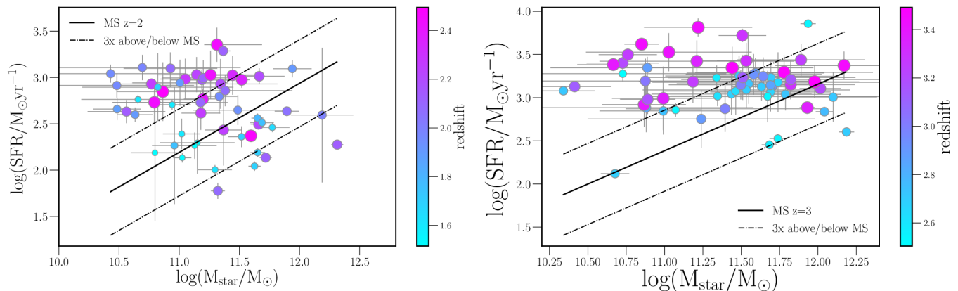
Fig. 9. Main sequence of galaxies. The black line shows the MS as defined in Speagle et al. (2014), with the dashed lines showing three times above and below the line of the MS for the redshift bin. The sources considered as starburst are three times above the MS. Left panel: The main sequence of galaxies for the redshift bin at 1.5 \leq z < 2.5 . In the z = 2 bin the fraction of starbursts with respect to the number of sources is 43%. Right panel: The main sequence of galaxies for the redshift bin at 2.5 \leq z < 3.5 . In the z = 3 bin the fraction of starbursts with respect to the number of sources is 40%. In both cases the starbursts tend to be of lower stellar mass than the majority of sources lying on the MS.
