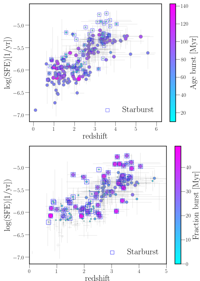
Fig. 11. SFE as a function of redshift. A general trend of increasing SFE with redshift is seen. This trend is more prominent in the starburst population (above the MS) identified by the blue border squares around the circles in the plot. Top-panel shows the dependence of the results on the age of the starburst (in the colour-bar). There is a clear dependence between the efficiency of star formation with the age of the starbursts: the later the starburst in the age of the galaxy the more efficient the star formation. The bottom-panel shows the same SFE-redshift plot with the dependence on the fraction of the star-formation burst (in the colour-bar), the more significant burst, the more efficient the star formation.
