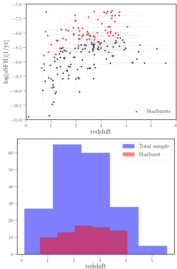
Fig. 8. (Top panel) Specific star-formation rate (sSFR) against redshift for the total sample. The galaxies classified as starbursts using the definition of Speagle et al. (2014) are marked as red dots and are seen to exhibit a higher sSFR than the rest of the population. (Bottom panel) Number-redshift distribution of the total sample (blue bars) and the starbursts (red bars). The fraction of starbursts increases up to z=2 , and it is similar out to z \sim 3-4 (around 40%), decreasing to higher redshifts z > 4 . A larger sample at z > 4 would be required to investigate the evolution of the starbursts over cosmic time.
