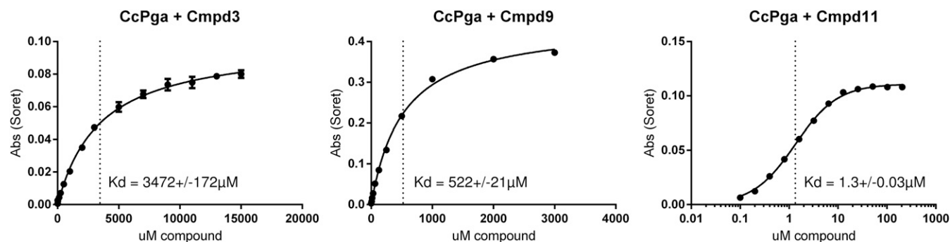
Fig. 4. Three representative ligand-binding curves. The Soret band shift is shown as a function of ligand concentration ( \mu M). The plots for compounds 3 and 9 are on a linear scale whereas, for clarity, the x axis of the plot for compound 11 is on the log scale. The dotted lines indicate the K_d . Circles and bars are the mean and estimated error of two observations, respectively.
