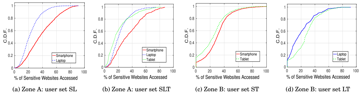
Fig. 11: Access of sensitive websites: percentage sensitive websites are maximum in smartphones - mainly due to social-networking, financial, education and email
