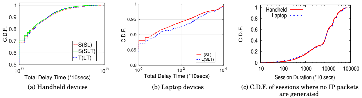
Fig. 9: a,b: Delay between IP assignment and usage - hand-held devices have a higher delay in creating the first packet after connection as compared to laptops. c: Distribution of sessions when no IP packets are created and the IP assignment is totally wasted.
