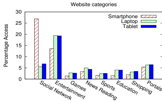
Fig. 6: Access of website categories in different device types: usage in laptops and tablets are almost the same and much different from smartphones.
