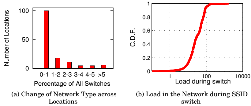
Fig. 15: Load and Location Dependence: Contributing factor in some cases, but not the major contribution for selection.
