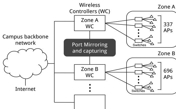
Fig. 1: Campus data capture setup
