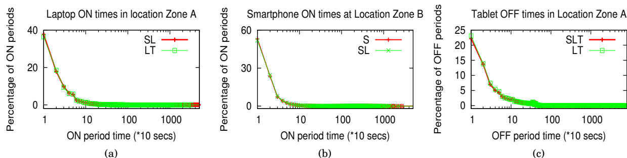
Fig. 8: “ON-OFF” period distributions: Intermittent network usage of the different device types is also independent of other user devices present
