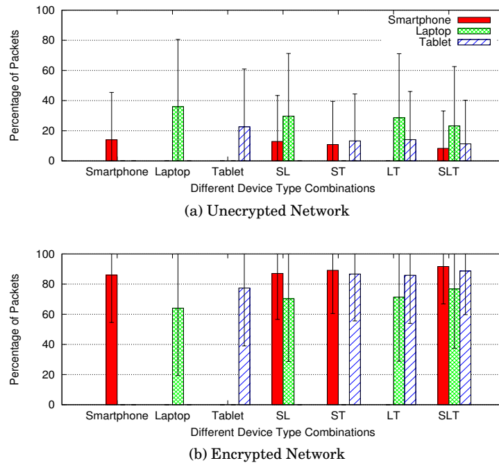
Fig. 14: Packets in encrypted and unencrypted network: In the unencrypted network, device behaviors are proportional to their screen size
