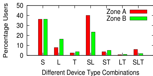
Fig. 3: Device Type Distributions at the two locations
