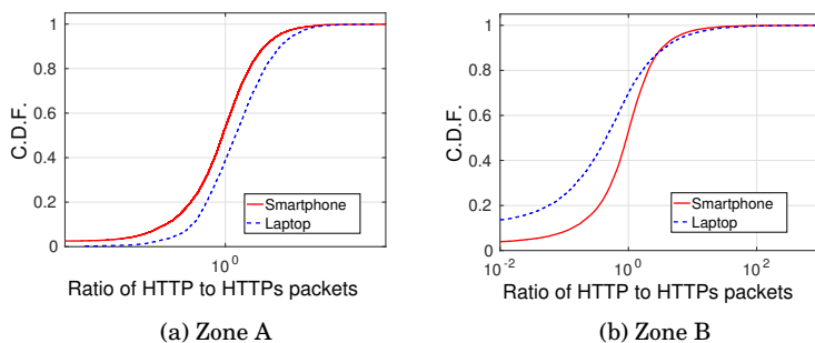
Fig. 12: Ratio of HTTP to HTTPS packets: The number of HTTP packets is higher in Zone A due to use of websites for videos, sports, news, etc.
