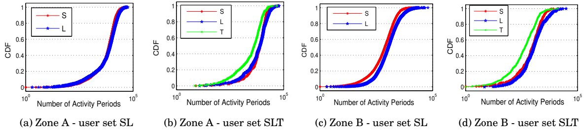
Fig. 4: Activity period distributions for user sets SL and SLT at zones A and B - the distributions remain the same for specific a device type of a user, irrespective of other user devices
