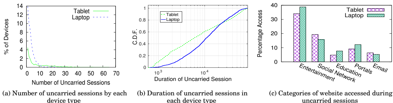
Fig. 10: Uncarried sessions: laptops create longer sessions, whereas tablets create shorter but more number of sessions. Most of the uncarried sessions are caused by media downloads or by syncing of social networking apps, emails, etc.
