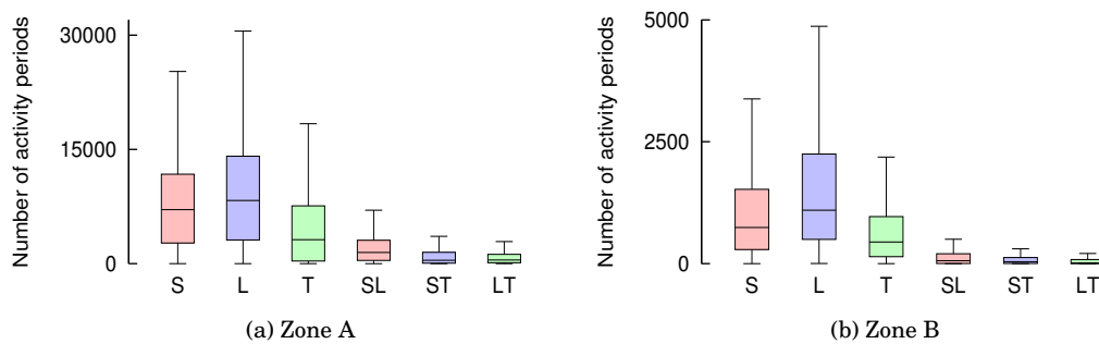
Fig. 7: Overlap of activity periods: overall very low overlap. Maximum overlap in smartphones and laptops
