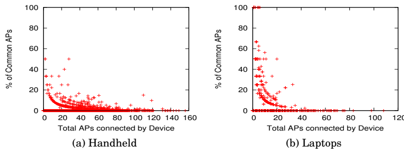
Fig. 16: Percentage of common access points
