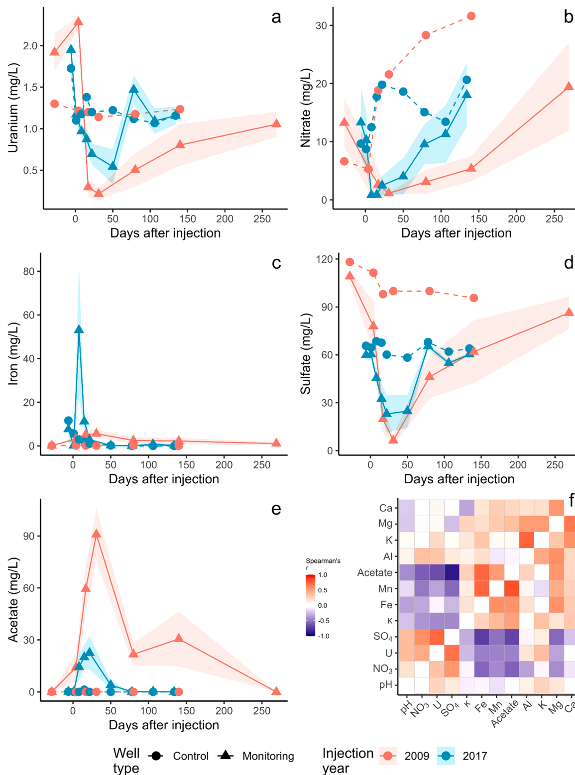
Fig. 1. Concentrations of selected geochemical species over the course of the injection and correlations between them. a) Uranium, \text{mgL}^{-1} . b) Nitrate, \text{mgL}^{-1} . c) Iron, \text{mgL}^{-1} . d) Sulfate, \text{mgL}^{-1} . e) Acetate, \text{mgL}^{-1} . f) Spearman's rank correlation coefficients between geochemical species in 2009 (upper triangle) and 2017 (lower triangle). a-e dashed lines and triangular points represent measurements from the control well. Shading represents \pm 1 standard error.
