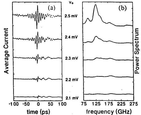
Figure 2. (a) Measured DC current induced in the junction by two incident picosecond electrical pulses which are separated by a time delay t . (b) Fourier transforms of the interference patterns.
