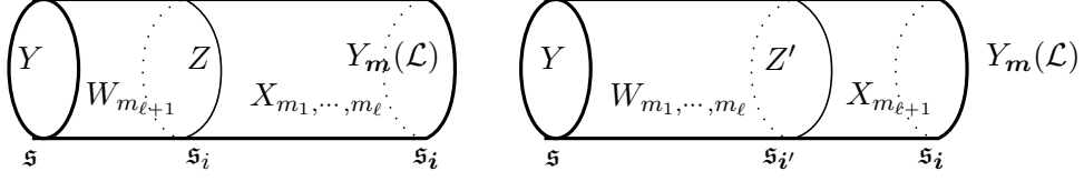
FIGURE 4. Two different decompositions of the two-handle cobordism W_{m_1, \dots, m_{\ell+1}} from Y to Y_m(\mathcal{L}) used in Lemma 5.10. The left cobordism consists of first attaching the two-handle to L_{\ell+1} and then attaching the remaining two-handles. The right cobordism consists of first attaching the two-handles along all components other than L_{\ell+1} and then attaching a two-handle along L_{\ell+1}
