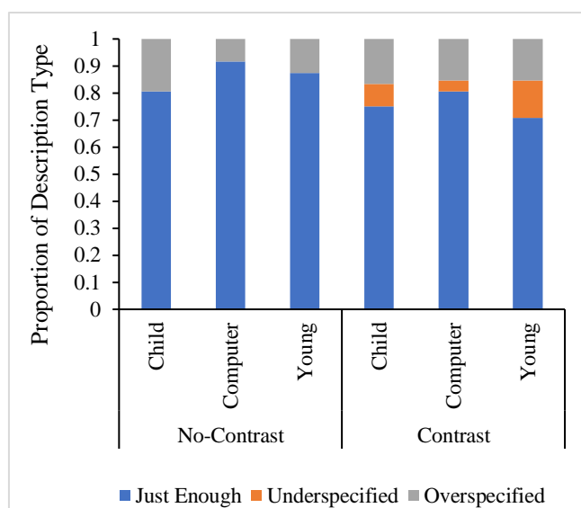
Figure 2. Informational adequacy by condition
