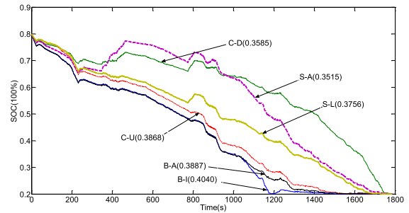
Fig. 12. SOC trajectories resulting from different control strategies.
