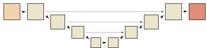
Fig. 2. A schematic representation of a common DCNN architecture with scaling operations. Downward arrows represent downscaling operations, upward arrows represent upscaling operations, and dashed arrows represent skip connections.
