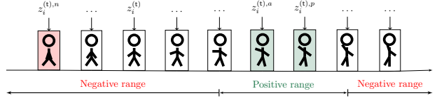
Figure 3: Triplet Condition in the transient latent space. Latent code representation of different frames of short video clips may lie very near to each other in the transient subspace. Using the proposed triplet condition, our model learns to explain the dynamics of similar looking frames and simultaneously map them to distinct latent vectors.
