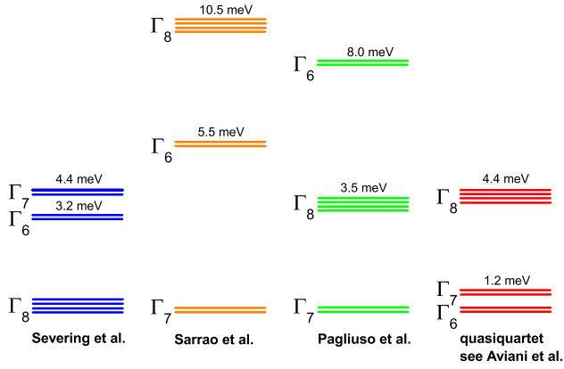
FIG. 1 (color online). Crystal-field schemes as published in [23–26].
