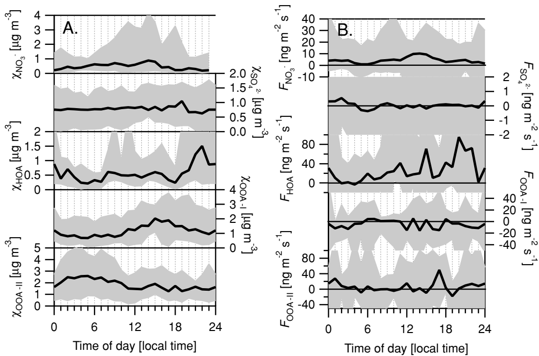
FIG. 16. Averaged diurnal cycles of chemically resolved particle concentrations and fluxes (FPEAK = -0.02).
