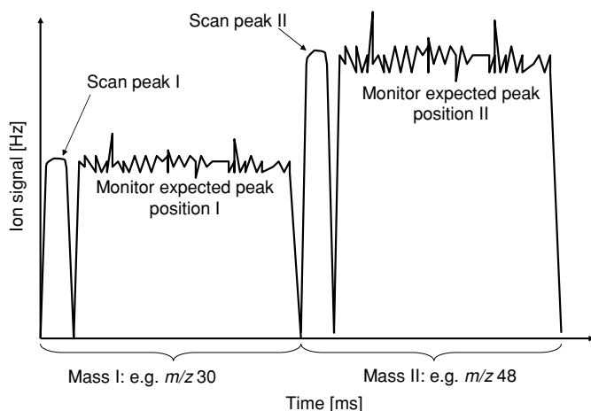
FIG. 2. Signal from the selective ion monitoring as implemented in the JMS mode (conceptual schematic). For each selected m/z , the instrument scans the peak and the settles on the anticipated peak position.
