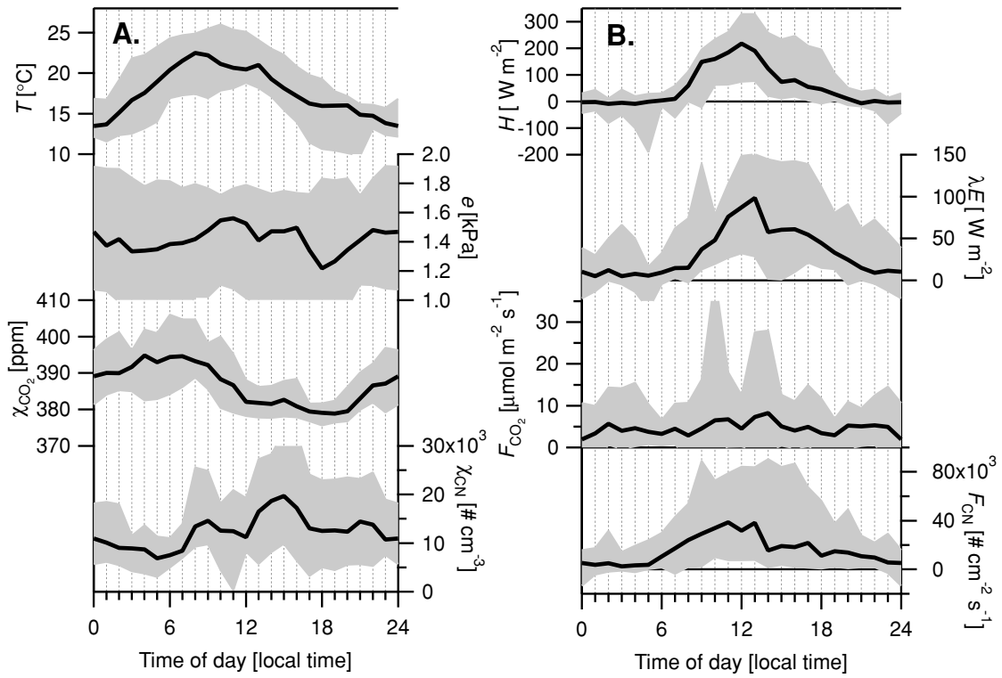
FIG. 15. (a) Averaged diurnal cycles of temperature ( T ), water pressure ( e ) and concentrations of CO 2 ( \chi_{CO_2} ) and small particles ( \chi_{CN} ). (b) Associated fluxes of sensible heat ( H ), latent heat ( \lambda E ), CO 2 ( F_{CO_2} ) and small particles ( F_{CN} ). Shown are medians (bold lines), together with range between 5th and 95th percentiles.
