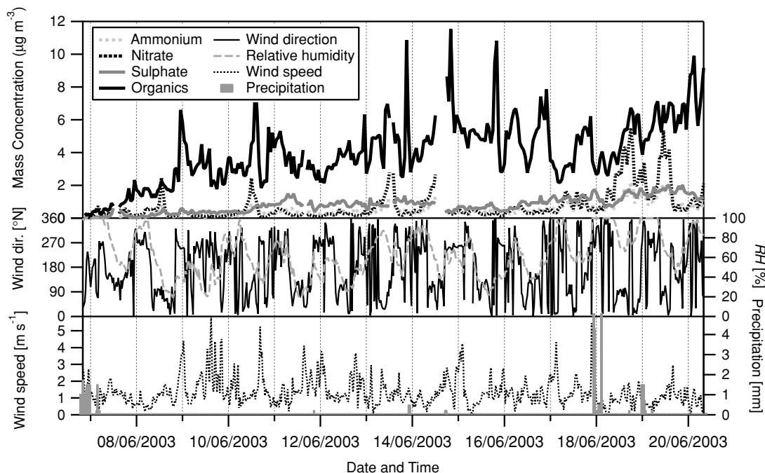
FIG. 8. Time-series of the 1 h average concentrations of non-refractory ammonium, nitrate, sulfate and total organics in \text{NR-PM}_{10} aerosol measured during the campaign in relation to meteorological variables ( RH and precipitation are taken from the Foothills weather station, http://www.atd.ucar.edu/weather/weather_fl/station.html , operated by NCAR/ATD).
