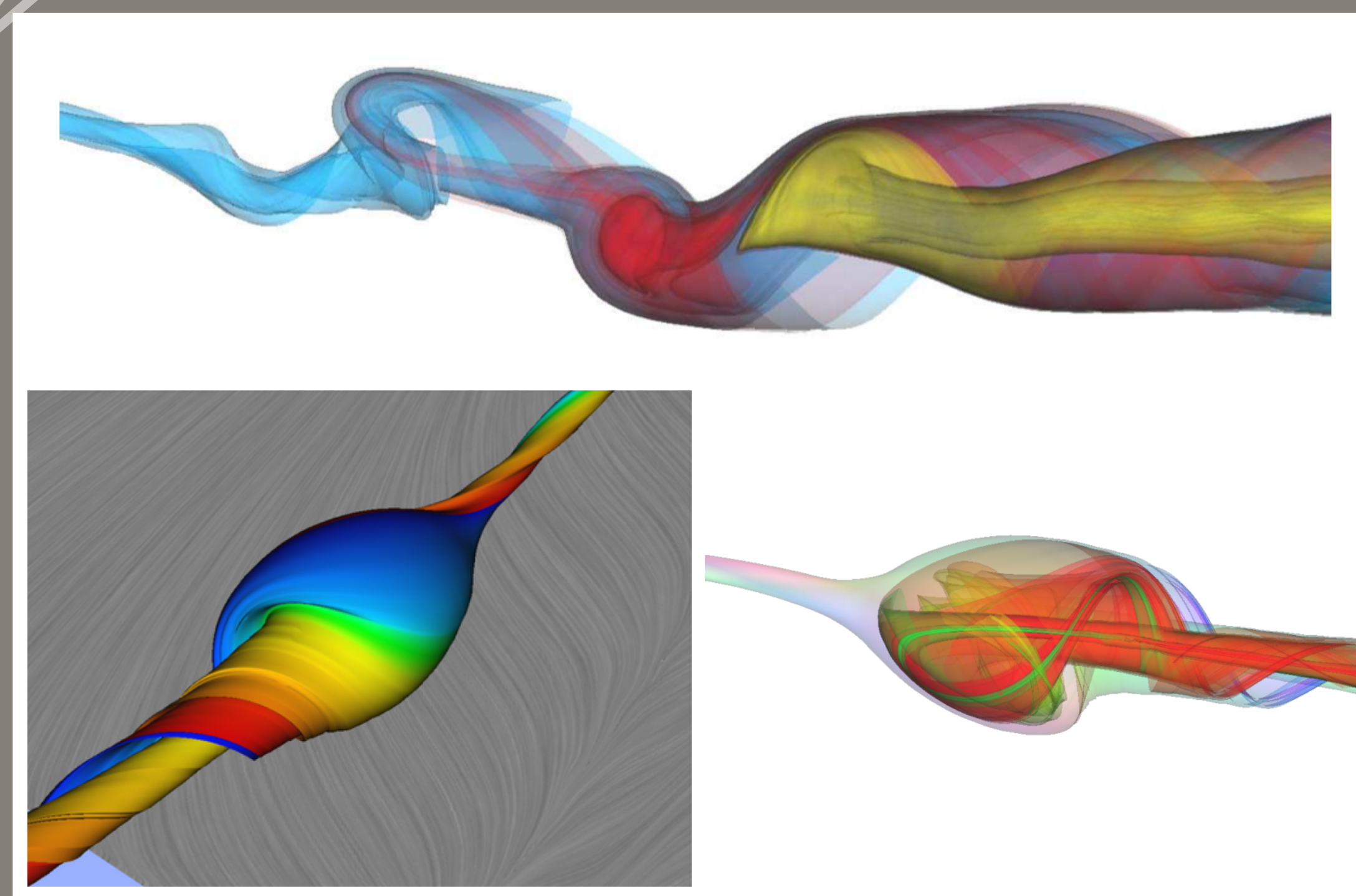
Top: Topological structure of a vortex breakdown in a simulation of a delta wing with low speed and high angle of attack. Stream surfaces in red and yellow show the separating surfaces emanating from two stagnation points that bound a so-called recirculation bubble.
