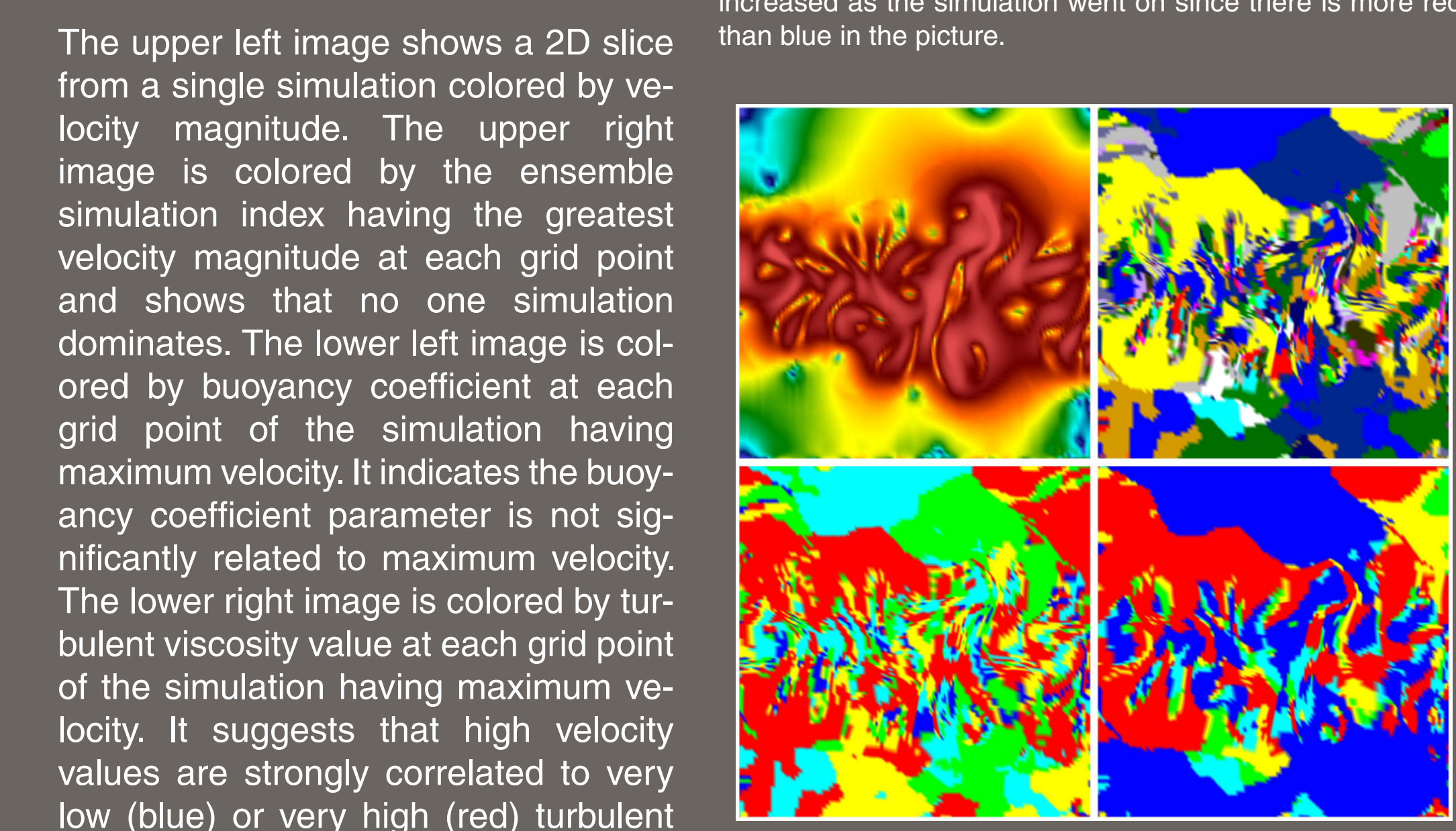
Figure 2: Visual and comparative analysis of results from an ensemble of Rayleigh-Taylor instability simulation runs. The objective is to understand the relationship between a subset of input parameters – turbulent viscosity and coefficient of buoyancy – and the resulting mixing rate.
