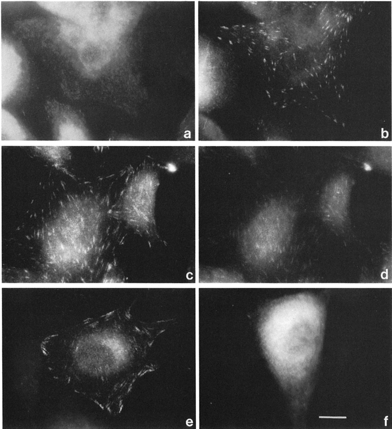
Figure 4. Ligand-binding independent recruitment of \alpha_{5b3}(\Delta 996)\beta_3 to focal adhesions. CHO cells were transfected and after 48 h were cultured on fibronectin substrates for 2 h. The cells were then stained with biotinylated anti-human \alpha_{5b3} (mAb PL98DF6) ( a , c , e , and f ) or anti-hamster \beta_1 (7E2) ( b and d ). The same cell was photographed in a , b , and c , d . The transfected integrins were \alpha_{5b3}\beta_3 ( a and b ), \alpha_{5b3}(\Delta 996)\beta_3 ( c and d ), \alpha_{5b3}(\Delta 996)\beta_3(D119\rightarrow Y) ( e ), and \alpha_{5b3}\beta_3(D119\rightarrow Y) ( f ). \alpha_{5b3}(\Delta 996) ( c ), but not wild-type \alpha_{5b3} ( a ), was detected at focal adhesions containing hamster \beta_1 . Ligand binding defective \alpha_{5b3}(\Delta 996)\beta_3(D119\rightarrow Y) was detected at focal adhesions in cells cultured on fibronectin ( e ), while \alpha_{5b3}\beta_3(D119\rightarrow Y) had a uniform cell surface distribution ( f ).
