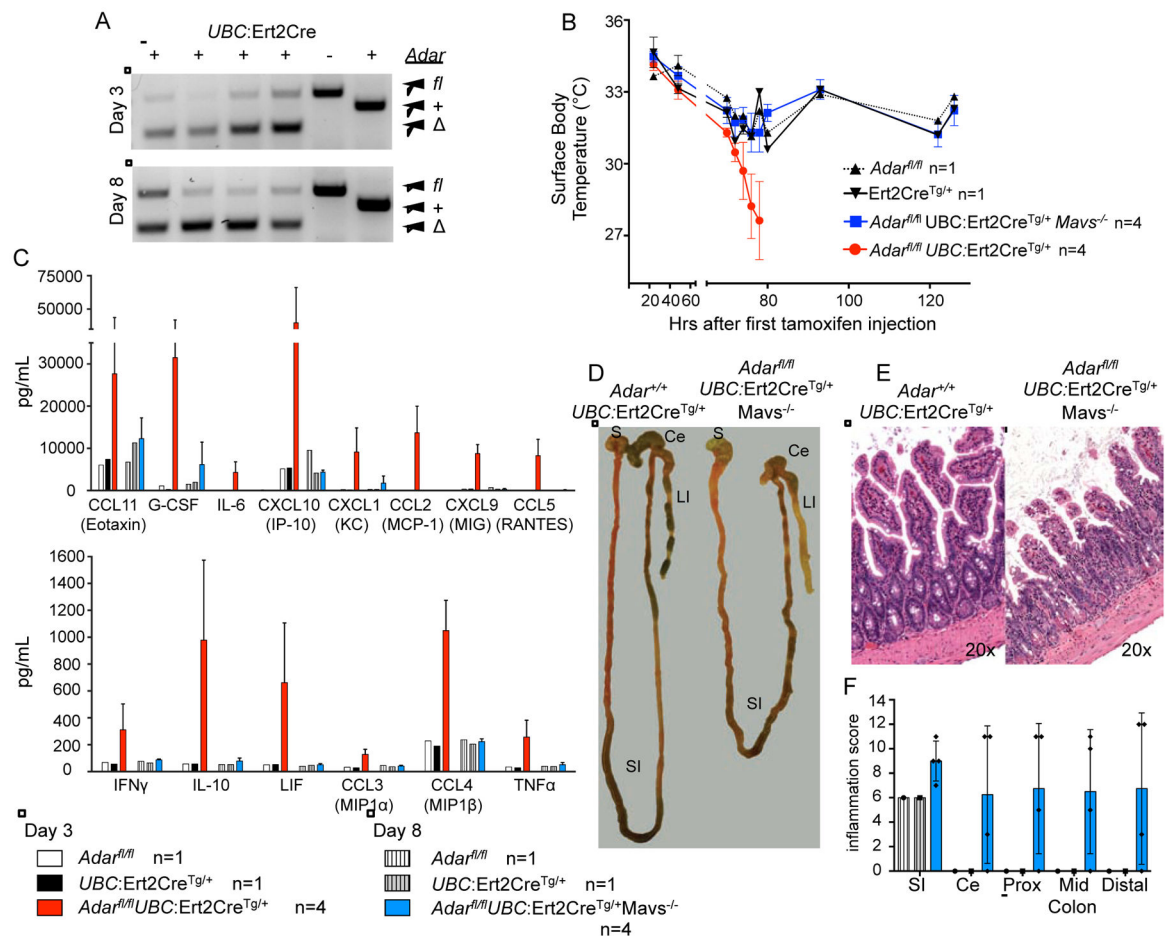
Figure 7. ADAR1 regulates both the MDA5-MAVS pathway and tissue homeostasis in adults Mice were treated with 2 mg tamoxifen i.p. daily for 3 days and observed for gross pathology.
