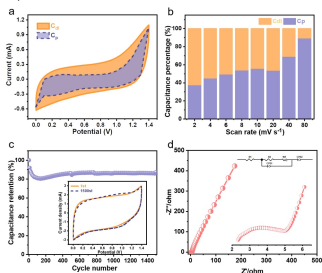
Figure 5. (a) Respective capacitance contribution of PAE-PcCo at scan rate of 2 mV s -1 . (b) Percentage of capacitance contribution at different scan rates. (c) Cycling stability test at 80 mV s -1 . Inset: comparison
