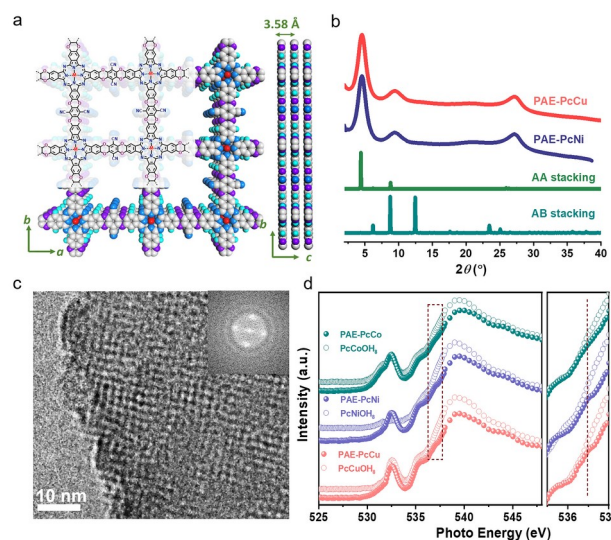
Figure 1. (a) Top ( ab plane) and side ( bc plane) view of the simulated crystal structure of PAE-PcCu with serrated AA stacking. (b) Experimental WAXS pattern for PAE-PcCu (red), PAE-PcNi (purple) and simulations based on serrated AA (green) and AB (dark cyan) stacking ( \lambda = 1.54 Å). (c) High resolution TEM images of PAE-PcCu. Inset: corresponding fast Fourier transform (FFT) result. (d) Oxygen K-edge XANES spectra for PAE-PcM and PcMOH 8 .
