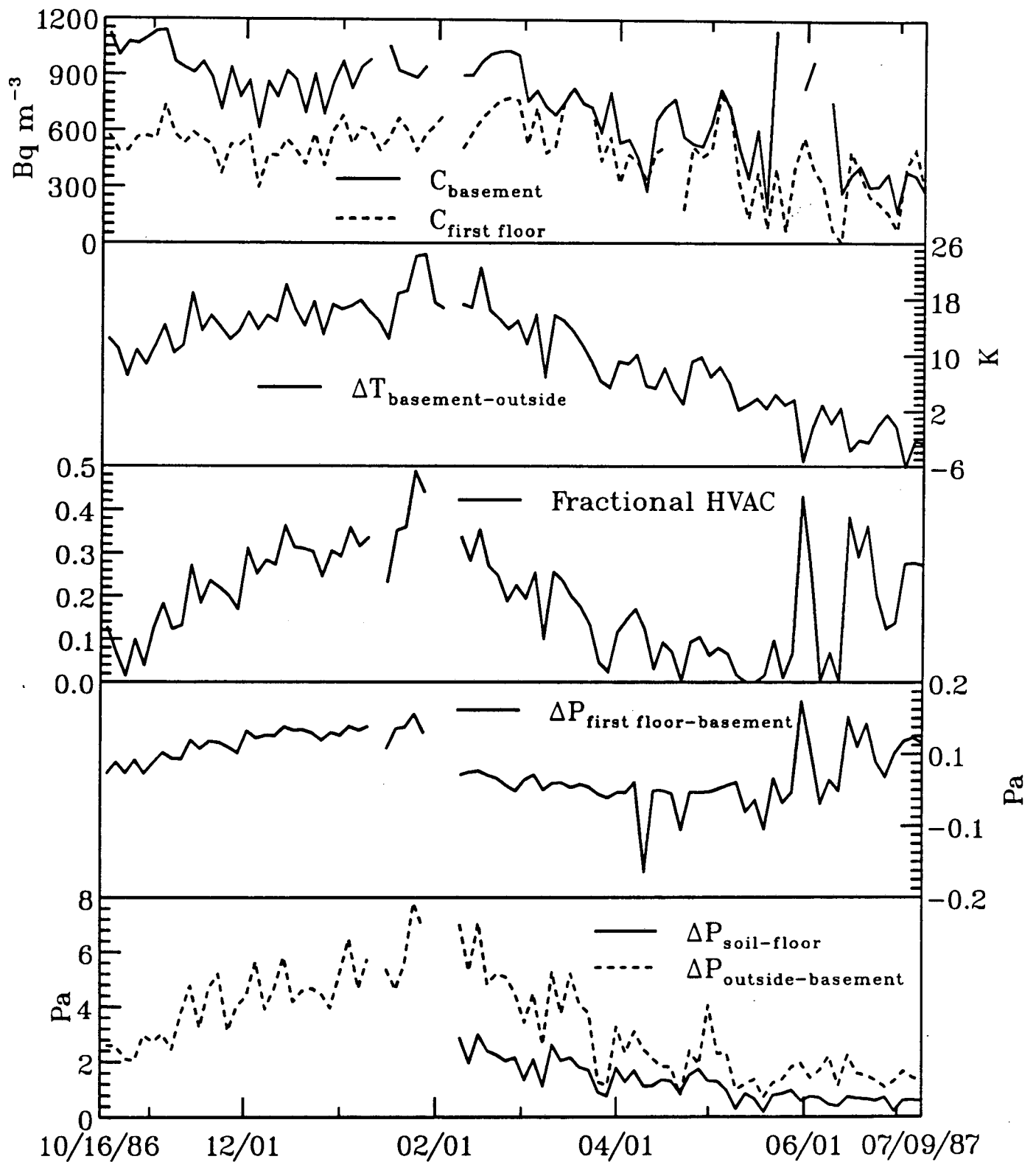
Figure 3. Radon concentrations and factors influencing those concentrations, House 2.
