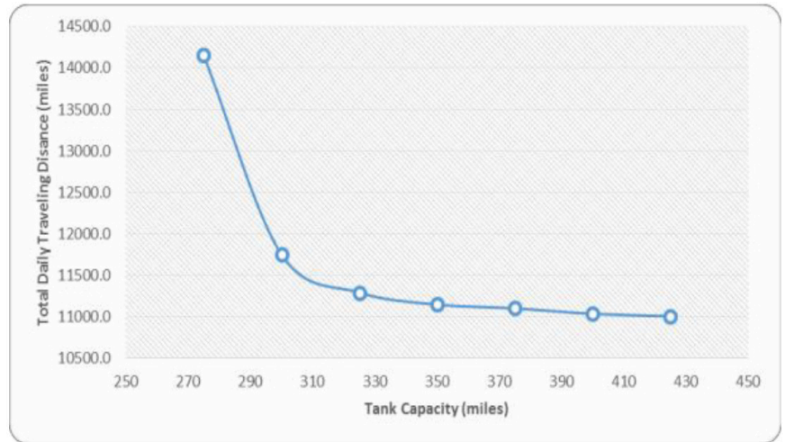
Figure 1. Total daily traveling distance with different tank capacities
