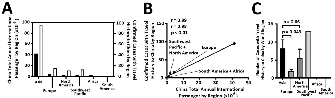
Figure 4. Distribution (A) and correlation (B) of international passenger numbers and global cases: Asia, Europe, North America, Southwest Pacific, Africa and South America. C) Medium number of cases and mean of the error for affected countries in each region as well as their respective case numbers.
