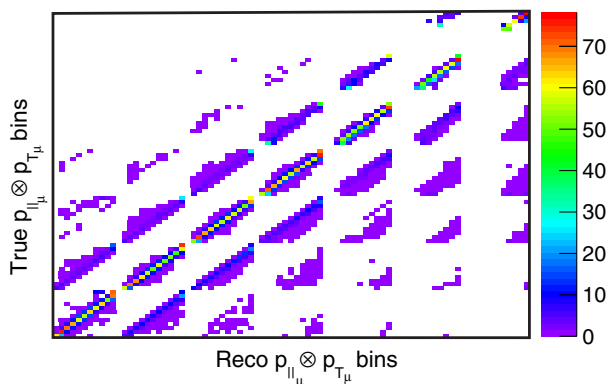
FIG. 10. Migration matrix for the p_{||} \otimes p_T distribution. The x axis corresponds to reconstructed bins, the y to true. The large cells correspond to p_T bins while the small cells are the p_{||} bins within a p_T bin. The high p_T overflow bin is included.
