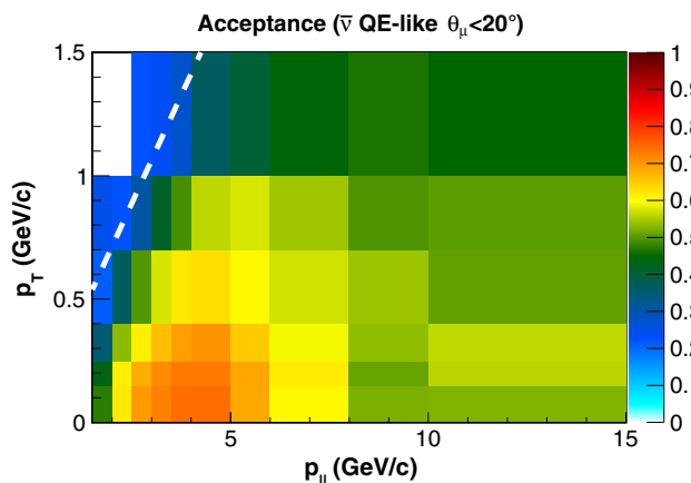
FIG. 11. Efficiency \times acceptance versus generated p_T and p_{||} , for QE-like events in the simulation. The dashed white line illustrates the 20^\circ limit imposed on reconstructed muon angles.
