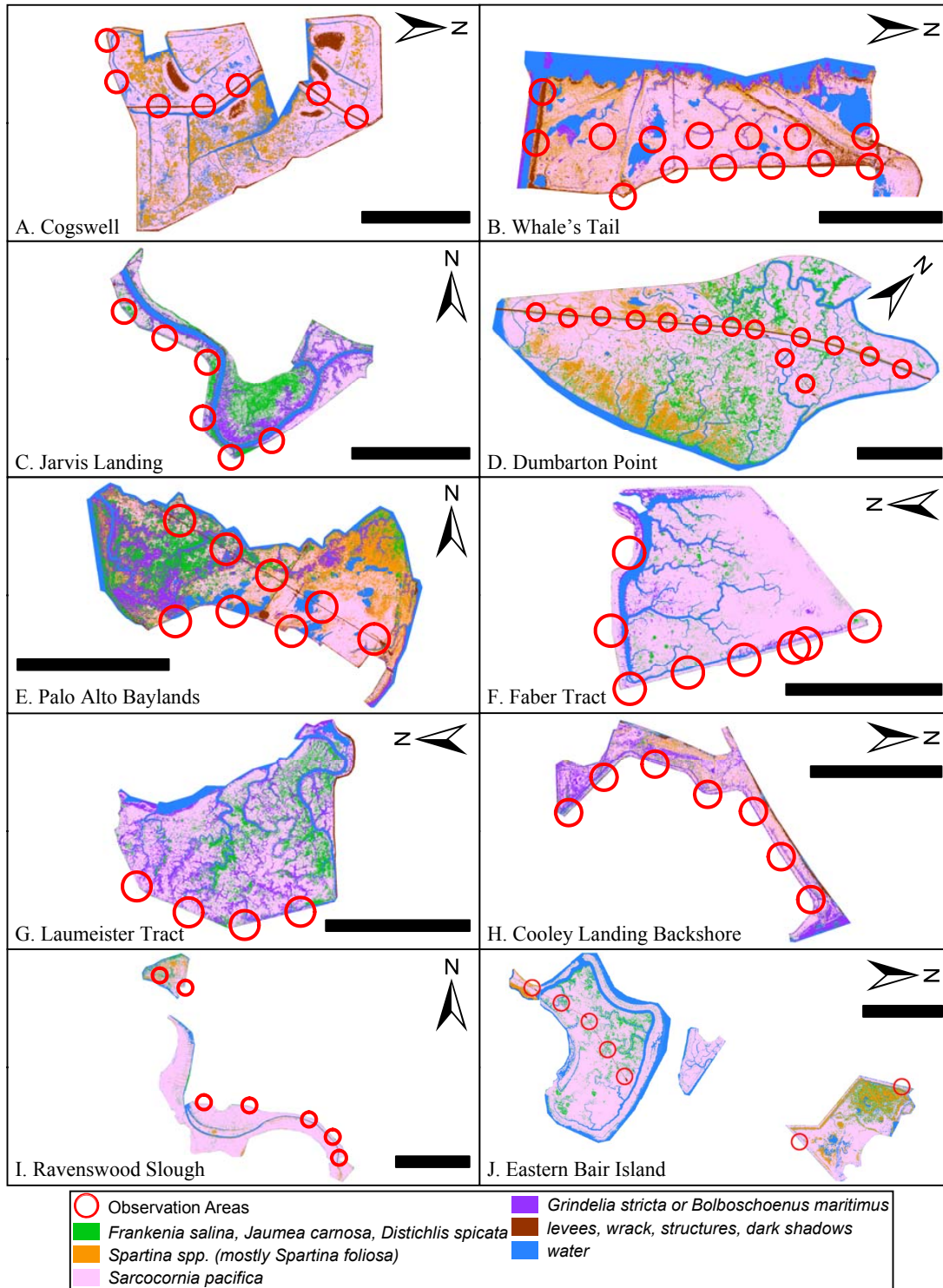
Figure 2 Classified marsh cover maps. Scale bars are 500-m long. Background imagery and larger versions of classified maps are provided in Appendix A.
