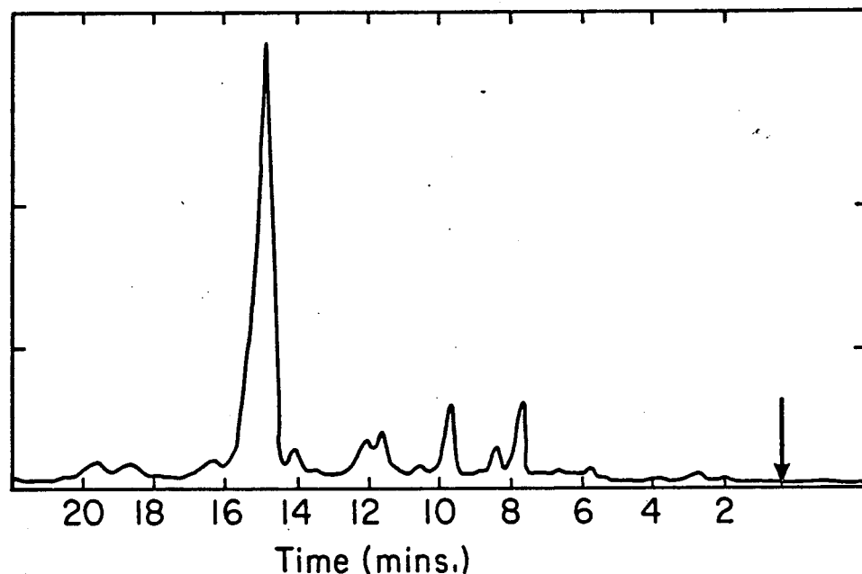
Fig. 1. HPLC trace of latex derived active fraction (ELA). Altex \text{C}_8 column. Mobile phase: \text{MeOH}:\text{H}_2\text{O} 1:1, Detection: 290nm.
