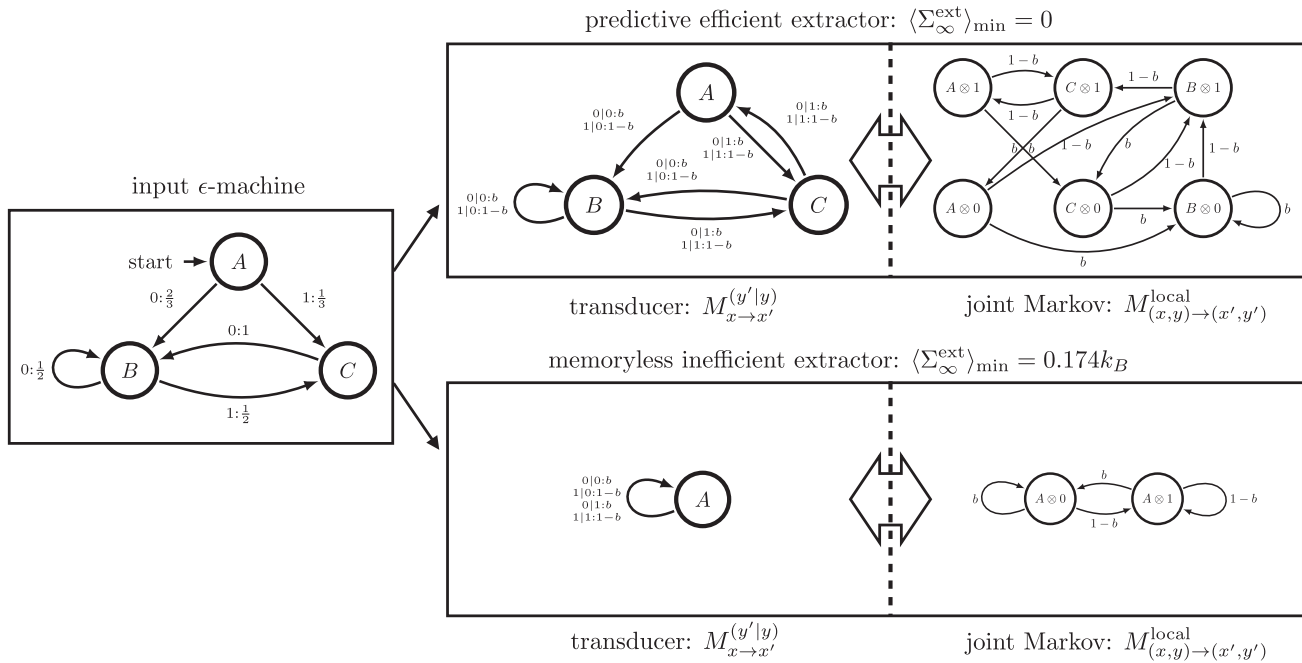
FIG. 4. Multiple ways to transform the golden mean process input, whose \epsilon -machine generator is shown in the far left box, into a sequence of uncorrelated symbols. The \epsilon -machine is a Mealy hidden Markov model that produces outputs along the edges, with y:p denoting that the edge emits symbol y and is taken with probability p . Top row: Ratchet whose internal states match the \epsilon -machine states and so it is able to minimize dissipation ( \langle \Sigma_{\infty}^{\text{ext}} \rangle_{\min} = 0 ) by making transitions such that the ratchet's states are synchronized to the \epsilon -machine's states. The transducer representation to the left shows how the states remain synchronized: Its edges are labeled y'|y:p , which means that, if the input is y , then the edge is taken with probability p and outputs y' . The joint Markov representation on the right depicts the corresponding physical dynamic over the joint state space of the ratchet and the interaction symbol. The label p along an edge from the state x \otimes y to x' \otimes y' specifies the probability of transitioning between those states according to the local Markov channel M_{(x,y) \rightarrow (x',y')}^{\text{local}} = p . Bottom row: In contrast to the efficient predictive ratchet, the memoryless ratchet shown is inefficient, since its memory cannot store the predictive information within the input \epsilon -machine, much less synchronize to it.
