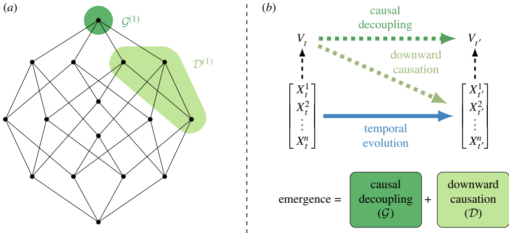
Figure 1. Schematic of the \Phi ID approach to causal emergence. (a) Lattice of \Phi ID information atoms, with atoms corresponding to causal decoupling ( \mathcal{G} ) and downward causation ( \mathcal{D} ) highlighted. (b) Relationship between system variables X_t , supervenient variables V_t and emergent properties (cf. equation (3.2)). Images adapted from [7,27,28]. (Online version in colour.)
