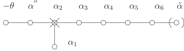
Figure 5: Extended Dynkin diagram of E_8 (III), and its maximal subalgebra \mathfrak{su}(3)_2 + \mathfrak{su}(2)_2 + \mathfrak{su}(6)_2 . \tilde{\alpha} \equiv 2L_0 - (L_1 + \dots + L_6) .
