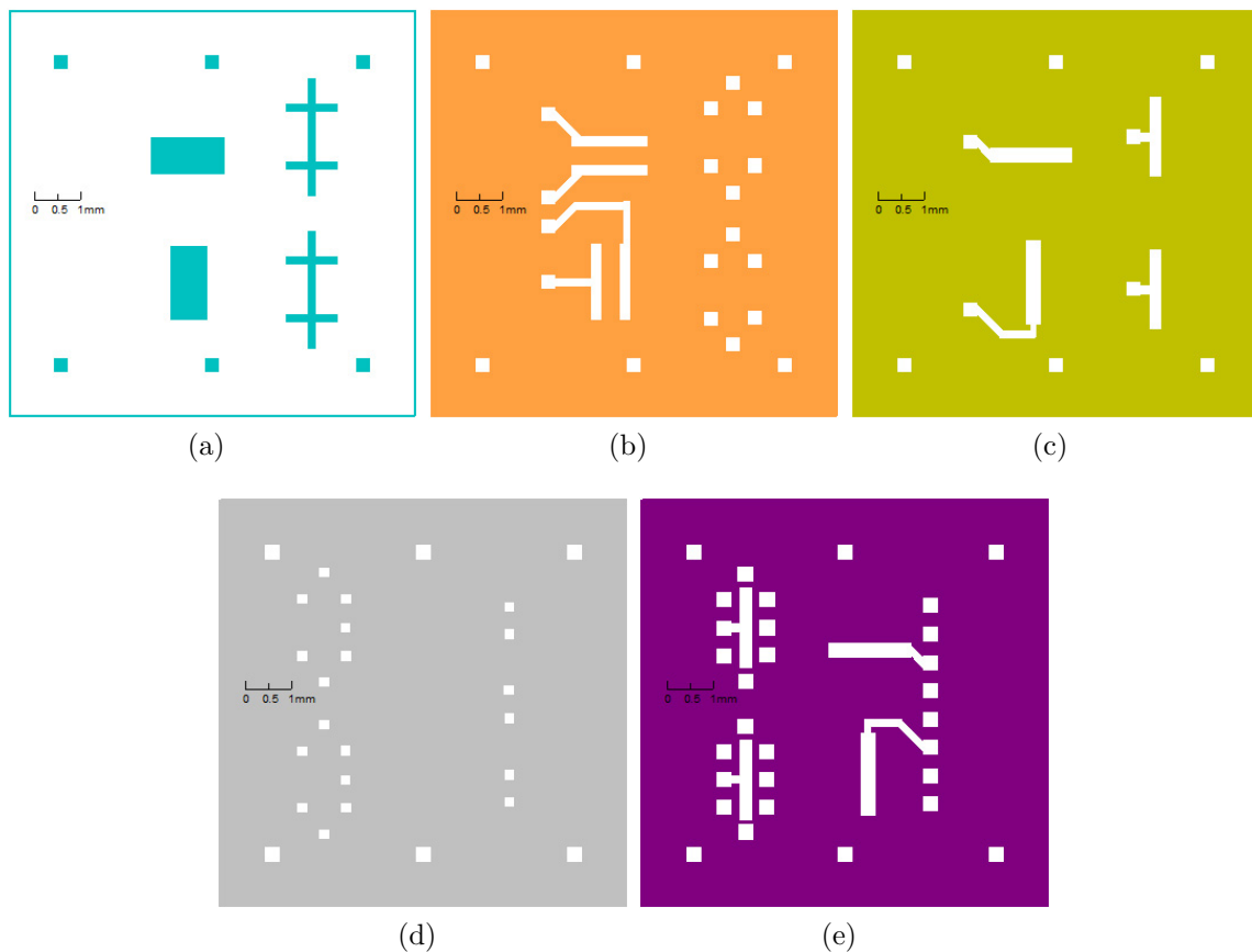
Figure A.8: A set of masks (a) mesa; (b) ohmic contacts; (c) front gate; (d) vias; (e) back gate and metal pads.
