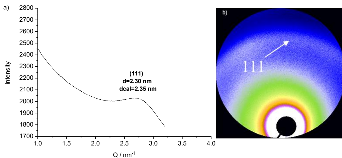
Figure S21. a) Synchrotron SAXS profile, and b) 2D image of Ru(BPY)_2(BDC)/WD-POM@SOF-1 powder crystals.
