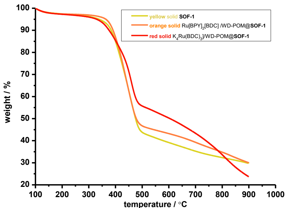
Figure S7. Thermogravimetric analysis of SOF-1 , K 4 Ru(BDC) 3 /WD-POM@SOF-1 and Ru(BPY) 2 (BDC)/WD-POM@SOF-1 that were obtained from slow evaporation, successive wash by methanol and water, and finally dried under vacuum.
