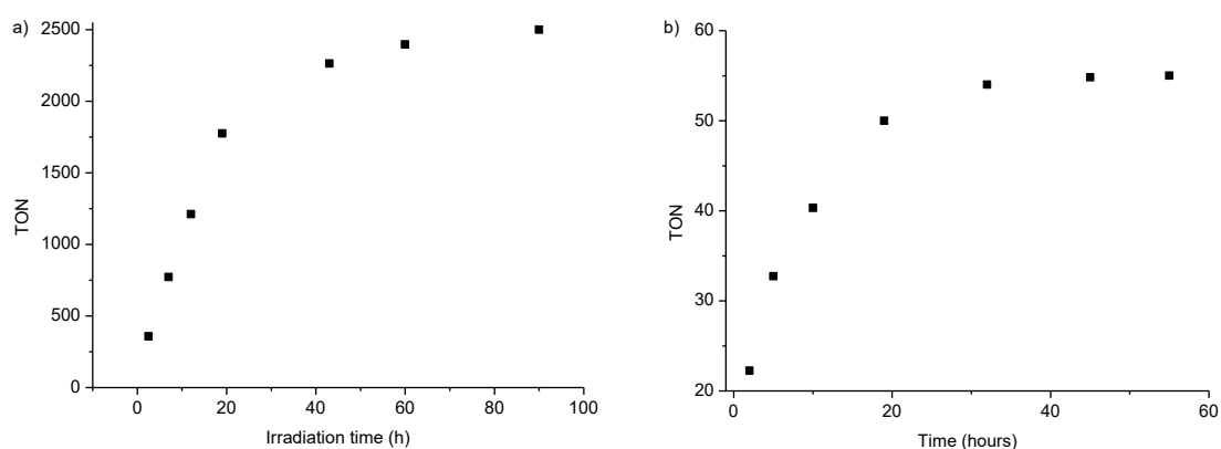
Figure S33. TON values of the H 2 generation systems vs irradiation time a) in the presence and b) absence of SOF-1 ([1] = 50 \mu\text{M} ) versus the irradiation time. The reaction system contained photosensitizer [Ru(BDC) 3 ] 4 (20 \mu\text{M} ), catalyst WD-POM (2 \mu\text{M} ), methanol (20 %, v/v) and pH = 1.8.
