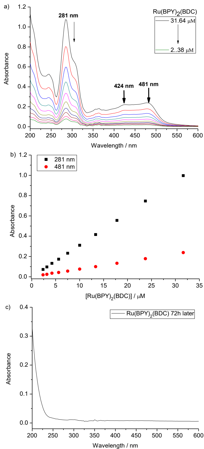
Figure S15. a) UV-Vis spectrum by gradual dilution, b) and the plots of the absorbance of guest Ru(BPY) 2 (BDC), c) the possible leaching of guest Ru(BPY) 2 (BDC) from the Ru(BPY) 2 (BDC)@SO \text{F} -1 hybrid after dialysis for 72h in water. The results indicated that the guest was absorbed by SO \text{F} -1 without leaching from the self-assembly hybrid.
