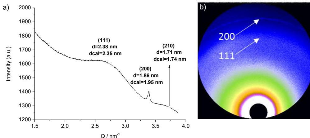
Figure S25. a) Synchrotron SAXS profile and b) 2D image of \text{K}_4\text{Ru}(\text{BDC})_3@ SOF-1 powder crystals.
