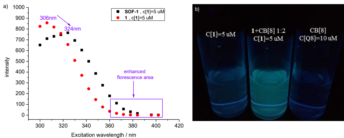
Figure S8. a) Enhanced fluorescence area of SOF-1 (1:CB[8] = 1:2, c[1]=5 M) compared with 1 , and b) its image seen by naked eyes under 365 nm light.
