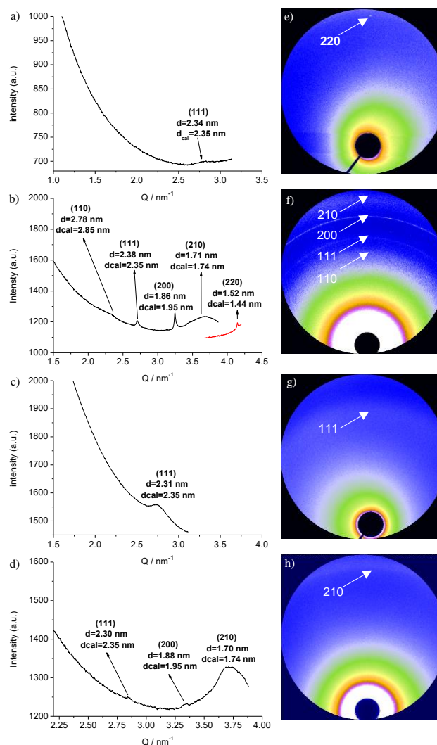
Figure 2. a) Solution-phase synchrotron SAXS profile of SOF-1 ( [1] = 2.0\text{mM} ) in water, b) solid-phase synchrotron SAXS profile of SOF-1 recorded separately for the same sample, and c) solid-phase synchrotron SAXS of SOF-1 after adsorbing \text{K}_4\text{Ru}(\text{BDC})_3 and WD-POM, d) solid-phase synchrotron SAXS of \text{K}_4\text{Ru}(\text{BDC})_3/\text{WD-POM}@ SOF-1 after 10-time repeated irradiation (19 h); e) and f) 2D synchrotron SAXS corresponding to profile b; g) 2D synchrotron SAXS corresponding to profile c; h) 2D synchrotron SAXS corresponding to profile d.
