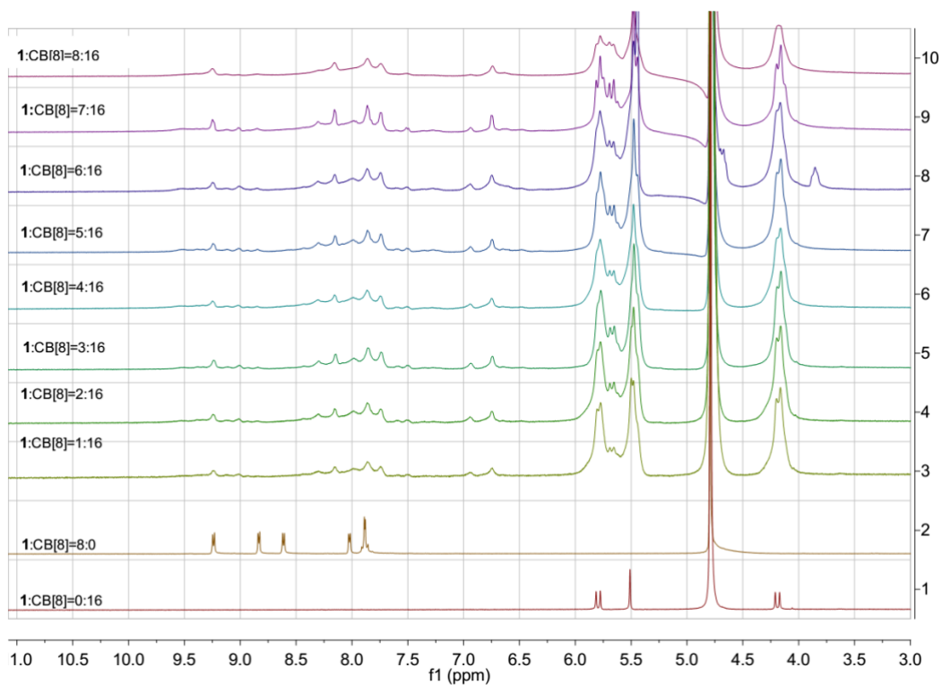
Figure S1. The ^1\text{H} NMR of gradual dissolution of CB[8] in \text{D}_2\text{O} with increasing amounts of molecule 1 (400 MHz, 25 °C, [\text{CB}[8]] = 2.0 \text{ mM} ). When 0.5 equiv. 1 added, the CB[8] dissolved completely.
