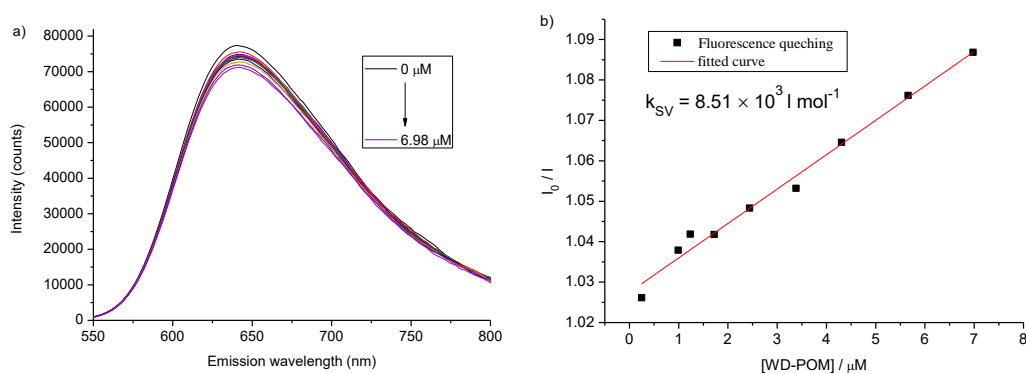
Figure S26. a) Steady-state emission quenching of \text{K}_4\text{Ru}(\text{BDC})_3 ( 20 \mu\text{M} ) by adding WD-POM ( 0 - 6.98 \mu\text{M} ) in the absence of SOF-1 with \lambda_{\text{ex}} = 460 \text{ nm} , \lambda_{\text{em}} = 627 \text{ nm} , b) and the corresponding quenching constants ( k_{\text{SV}} ) fitted by Stern-Volmer equation (red line). Conditions: \text{K}_4\text{Ru}(\text{BDC})_3 ( 20 \mu\text{M} ), MeOH ( 20 \% v/v), \text{pH} = 1.8 , WD-POM ( 2 \mu\text{M} ).
