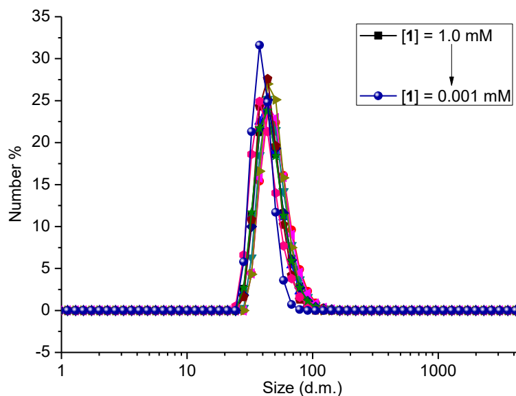
Figure S5. The of DLS result of SOF in water at 25 °C varied concentrations of 1 from 1.0 mM to 0.001 mM. The stable hydrodynamic diameters indicated the stability of SO F-1 at different concentrations. All the samples were measured after being left to stand for 48 hours.
