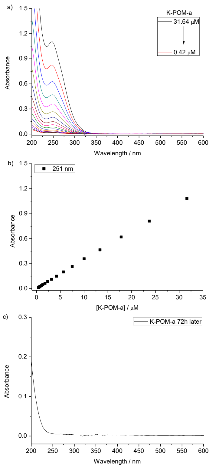
Figure S17. a) UV-Vis spectrum by gradual dilution, b) the plots of the absorbance of guests K-POM-a, c) the possible leaching of guests K-POM-a from the K-POM-a @SO F -1 hybrid after dialysis for 72h in water. The results indicated that the guest was absorbed by SO F -1 without leaching from the self-assembly hybrid.
