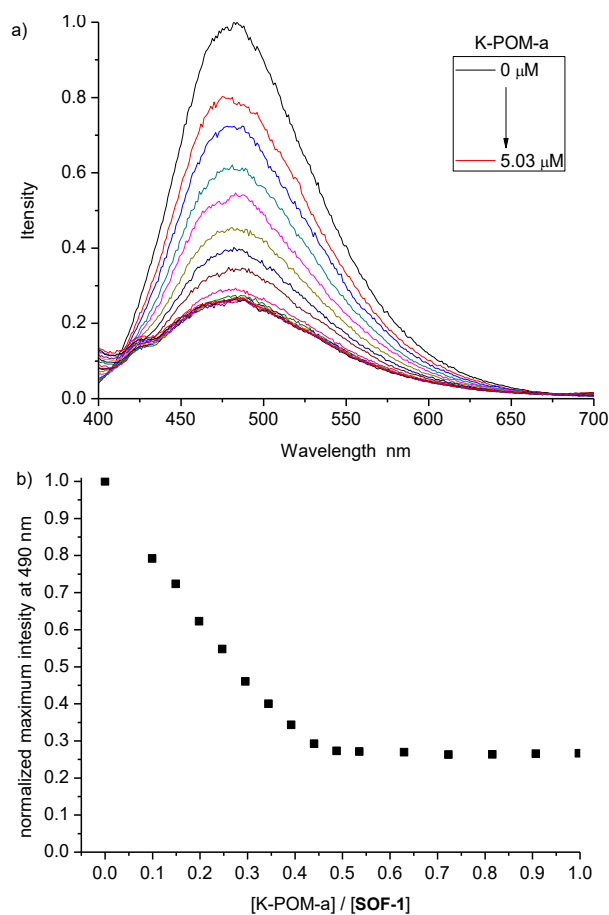
Figure S12. Fluorescence quenching of SOF-1 ( [1]=5 \mu\text{M} ) at the excitation of 370 nm by adding guest K-POM-a (0-5.03 \mu\text{M} ).
