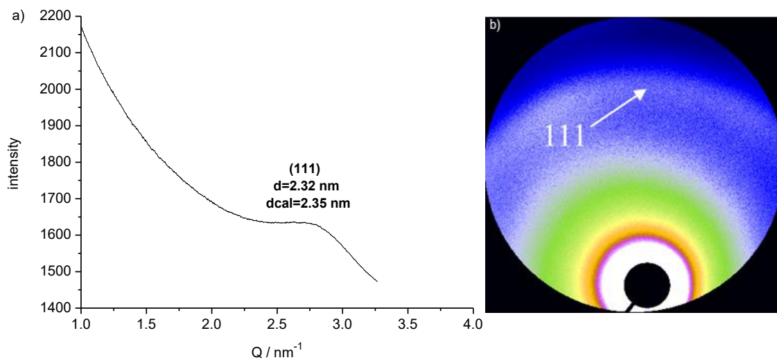
Figure S20. a) Synchrotron SAXS profile, and b) 2D image of K_4Ru(BDC)_3/K-POM-a@SOF-1 powder crystals.
