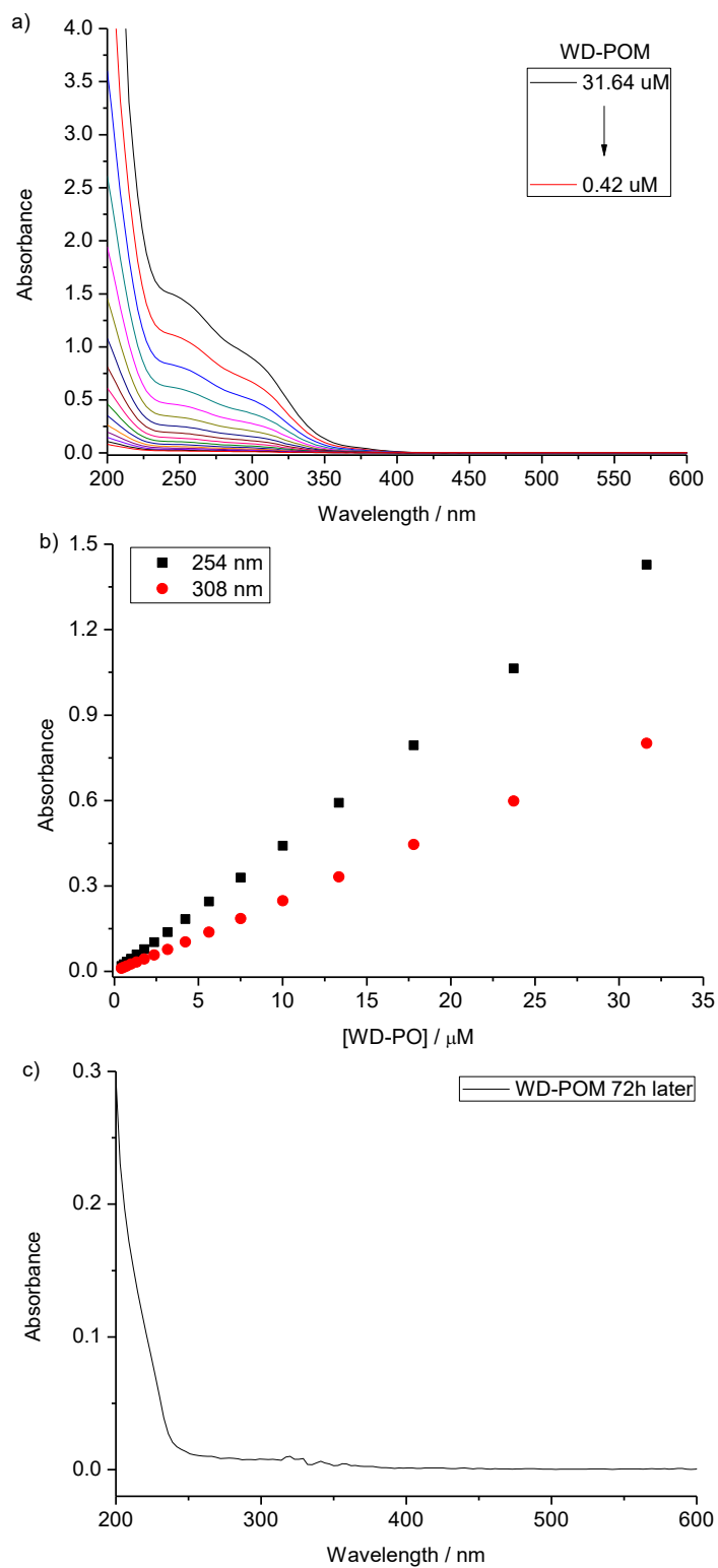
Figure S16. a) UV-Vis spectrum by gradual dilution, b) and the plots of the absorbance of guests WD-POM, c) the possible leaching of guests WD-POM from the WD-POM@ SO F-1 hybrid after dialysis for 72h in water. The results indicated that the guest was absorbed by SO F-1 without leaching from the self-assembly hybrid.
