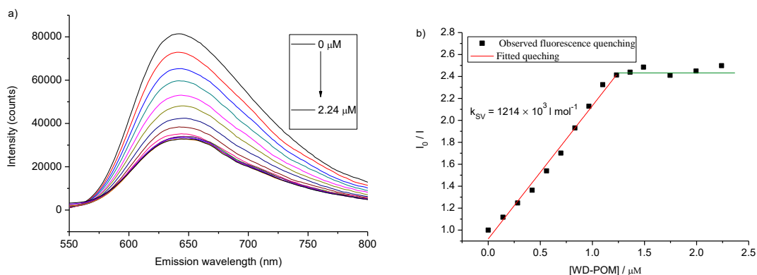
Figure S27. a) Steady-state emission quenching of \text{K}_4\text{Ru}(\text{BDC})_3 ( 20 \mu\text{M} ) by adding WD-POM ( 0 - 2.24 \mu\text{M} ) in the presence of SOF-1 ( [\text{I}] = 50 \mu\text{M} ) with \lambda_{\text{ex}} = 460 \text{ nm} , \lambda_{\text{em}} = 627 \text{ nm} , b) and the corresponding quenching constants ( k_{\text{SV}} ) fitted by Stern-Volmer equation (red line). Conditions: \text{K}_4\text{Ru}(\text{BDC})_3 ( 20 \mu\text{M} ), MeOH ( 20 \% v/v), \text{pH} = 1.8 , WD-POM ( 2 \mu\text{M} ).
