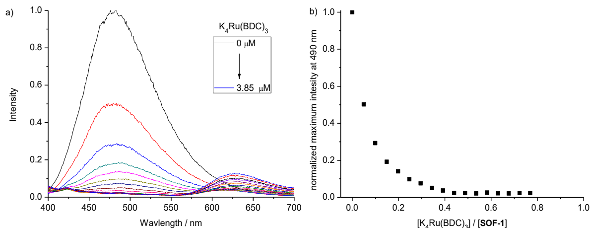
Figure S9. Fluorescence quenching of SOF-1 ( [1]=5 \mu\text{M} ) at the excitation of 370 nm by adding guest \text{K}_4\text{Ru}(\text{BDC})_3 (0-3.85 \mu\text{M} ).
