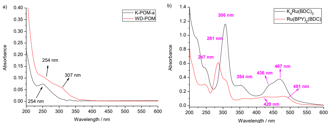
Figure S32. UV-Vis spectrum of the WD-POM and K-POM-a (2 \mu\text{M} ), and b) K 4 Ru(BDC) 3 and Ru(BPY) 2 (BDC) (20 \mu\text{M} ) in water.
