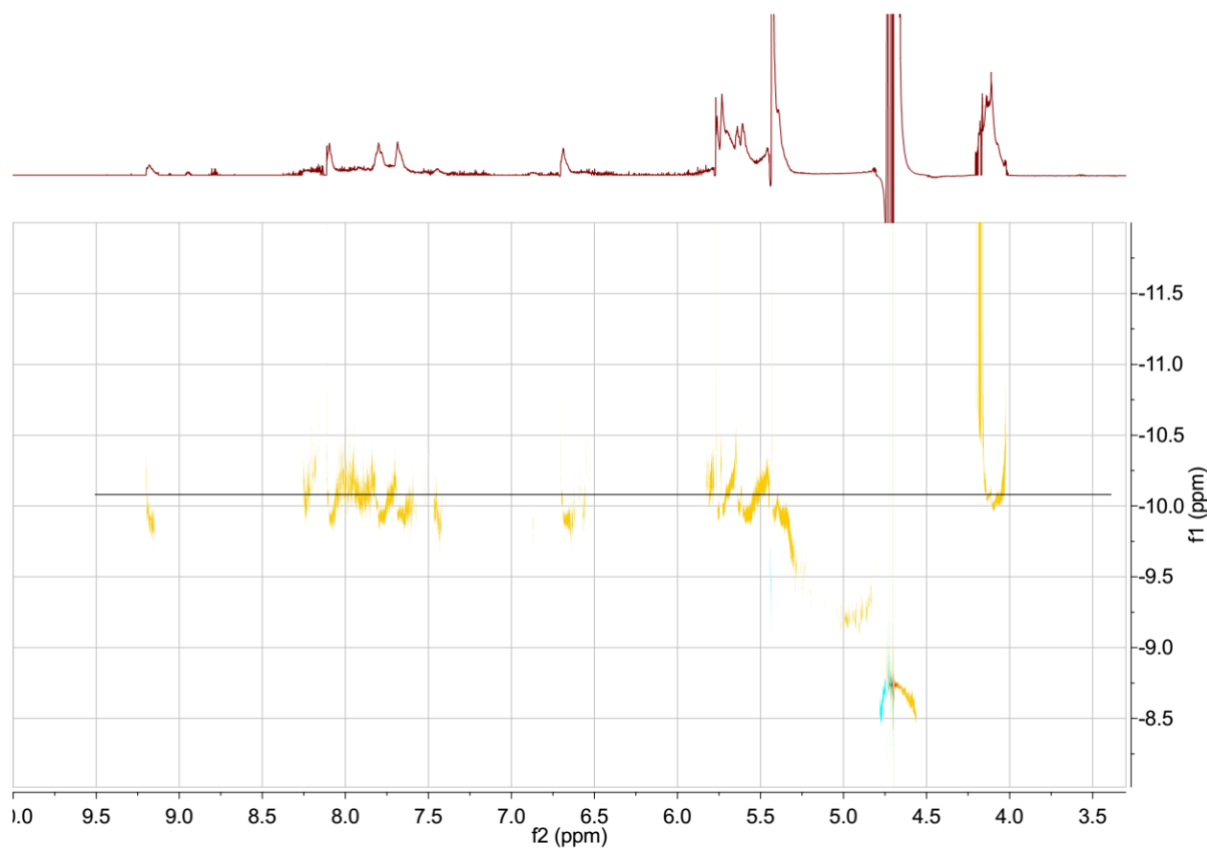
Figure S24. DOSY ^1\text{H} NMR spectrum (400 MHz) of the mixture of SOF-1 ( [\mathbf{1}]=1.0 mM), \text{K}_4\text{Ru}[\text{BDC}]_3 (0.2 mM) and WD-POM (0.02 mM) in \text{D}_2\text{O} showed similar peaks with a series of noise which be attributed to the adding of \text{K}_4\text{Ru}(\text{BDC})_3 and WD-POM . The ordinate represents the log value of the diffusion constant. Note: this spectrum was obtained from the former sample by adding \text{K}_4\text{Ru}(\text{BDC})_3 and WD-POM .
