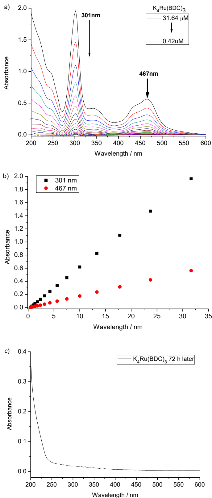
Figure S14. a) UV-Vis spectrum by gradual dilution, b) the plots of the absorbance of guest K_4Ru(BDC)_3 , c) and the possible leaching of guest K_4Ru(BDC)_3 from the K_4Ru(BDC)_3 @SOF-1 hybrid after dialysis for 72h in water. The results indicated that the guest was absorbed by SOF-1 without leaching from the self-assembly hybrid.
