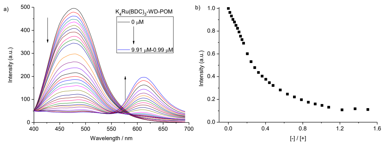
Figure S13. Fluorescence quenching of SOF-1 ( [1]=5 \mu\text{M} ) at the excitation of 370 nm by adding guest K 4 Ru(BDC) 3 /WD-POM (0-9.91/0.99 \mu\text{M} ).
