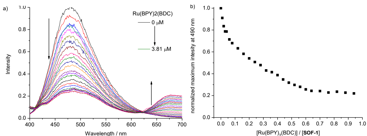
Figure S10. Fluorescence quenching of SOF-1 ( [1]=5 \mu\text{M} ) at the excitation of 370 nm by adding guest \text{Ru}(\text{BPY})_2(\text{BDC}) (0-3.81 \mu\text{M} ).
