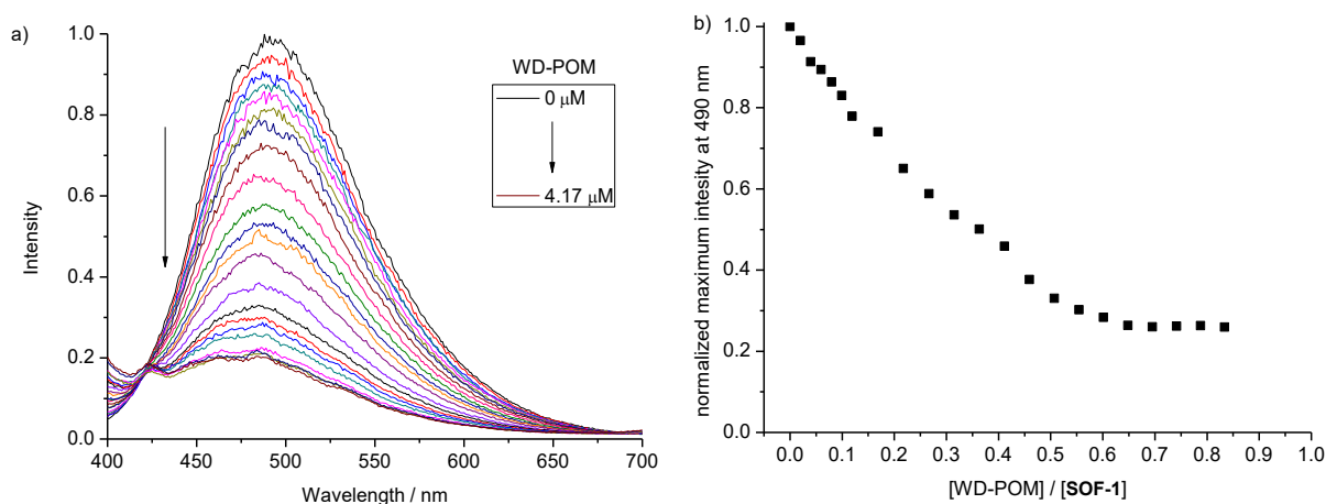
Figure S11. Fluorescence quenching of SOF-1 ( [1]=5 \mu\text{M} ) at the excitation of 370 nm by adding guest WD-POM (0-4.17 \mu\text{M} ).
