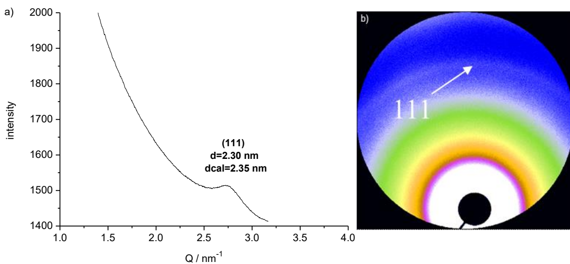
Figure S22. a) Synchrotron SAXS profile and b) 2D image of Ru(BPY)_2(BDC)/K-POM-a@SOF-1 powder crystals.
