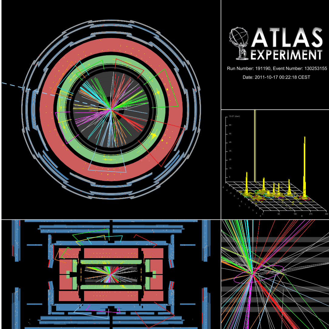
Figure 8. A display of an event which passes the 9j55 and 7j80 signal region selections. The event has E_T^{\text{miss}}/\sqrt{H_T} of 4.1 \text{ GeV}^{1/2} , H_T of 1.47 \text{ TeV} and E_T^{\text{miss}} of 157 \text{ GeV} .
