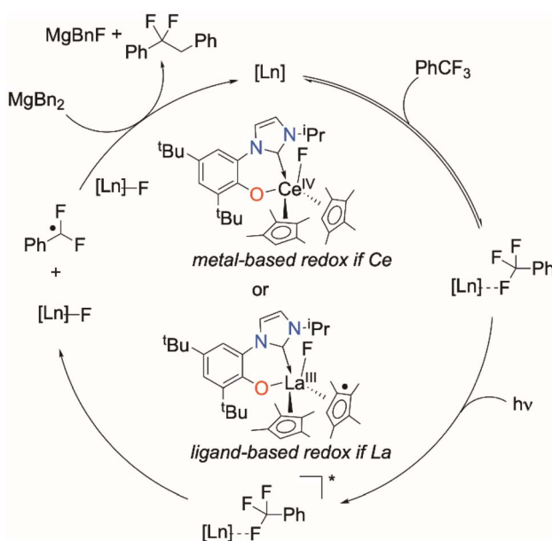
Scheme 7 Proposed mechanism of photocatalytic C–C coupling.
