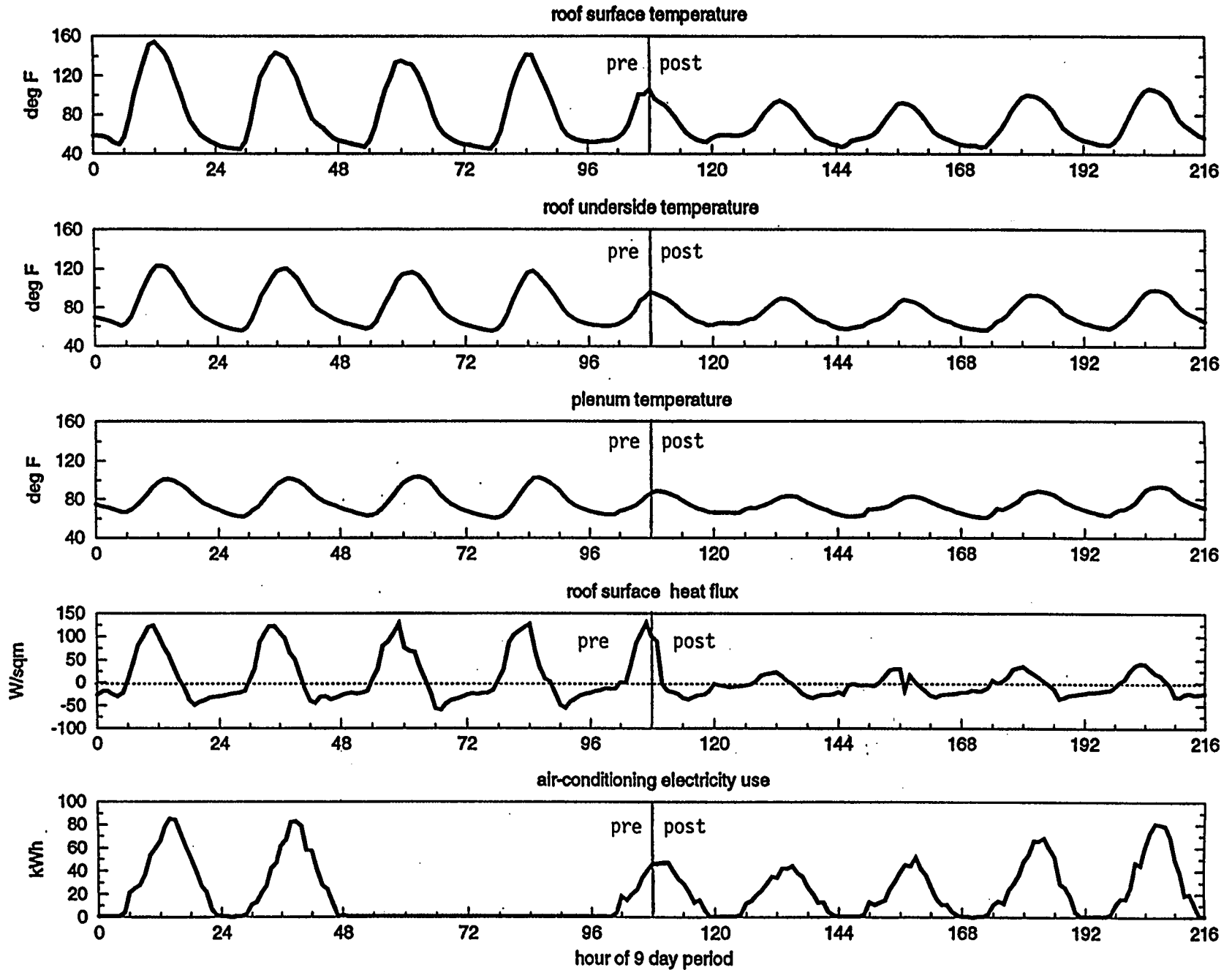
Figure 1. Gilroy monitored hourly data: 8/1-8/9/96.
