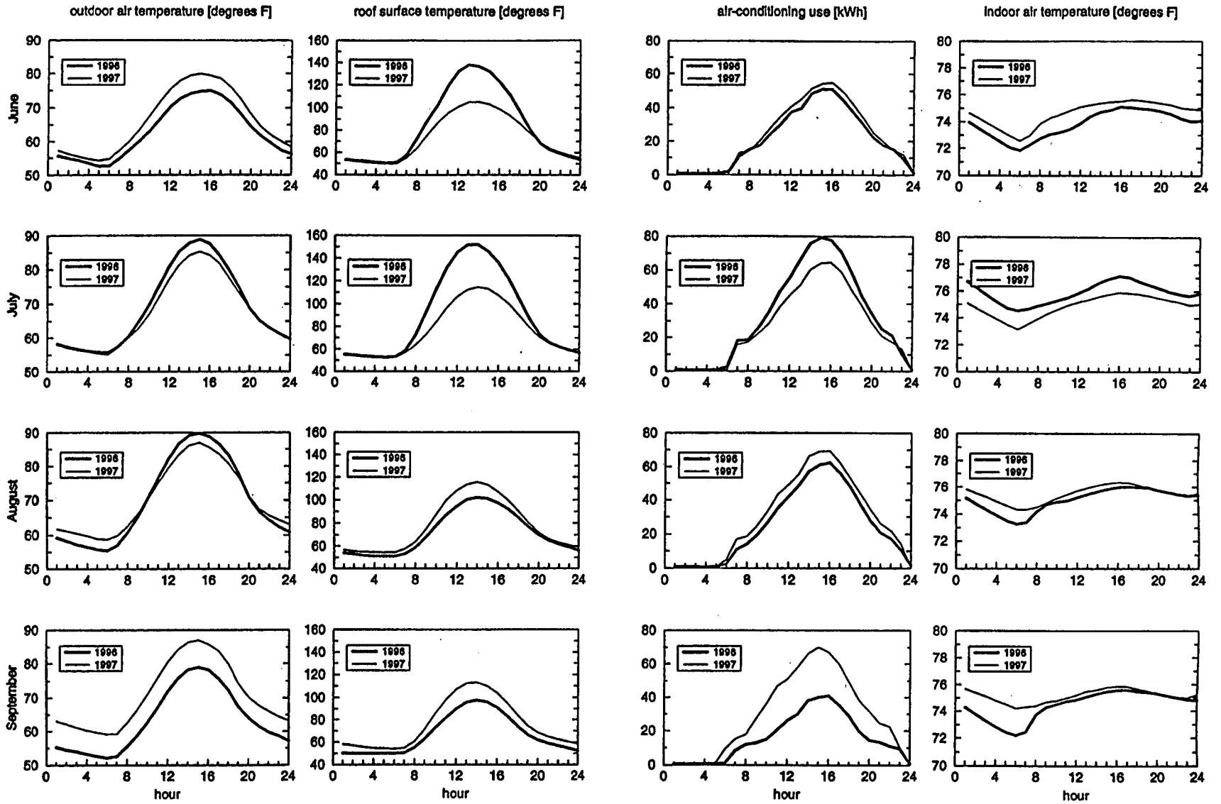
Figure 2. Gilroy average standard weekday profiles of outdoor air, indoor air, and roof surface temperatures, and a/c electricity use for June, July, August, and September 1996 and 1997.
