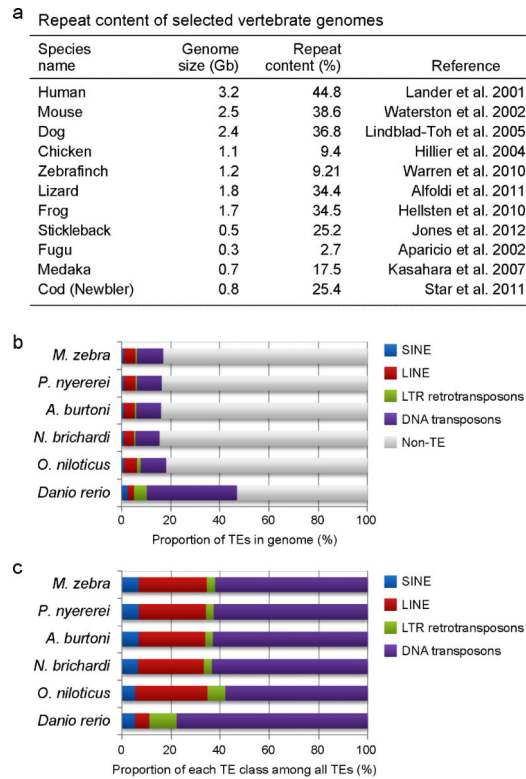
Extended Data Figure 5. Comparison of TEs among cichlids and other vertebrate genomes a , Repeat content of selected vertebrate genomes. Table, no legend. b , Proportions of TEs in the genomes. c , Proportions of each TE class among all TEs. The TE proportions are much lower in cichlid genomes than that in zebrafish.
