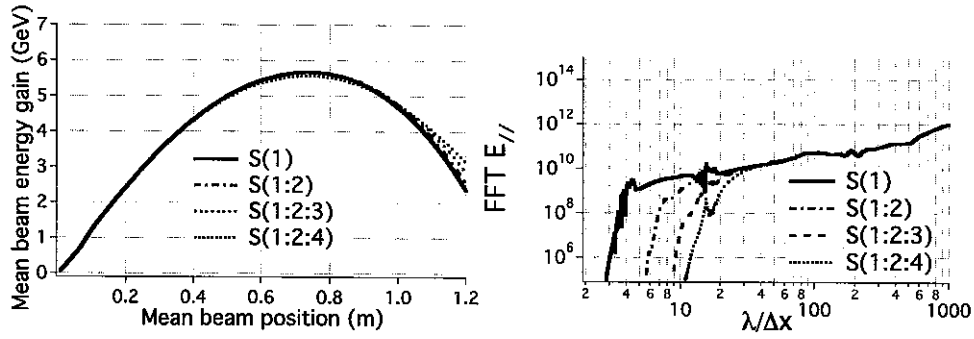
Figure 21: (left) Average beam energy gain versus longitudinal position (in the laboratory frame), (right) Fourier Transform of the longitudinal electric field at t=40 ps, averaged over whole domain, from 3D simulations of a full scale 10GeV LPA in a boosted frame at \gamma = 130 , using the CK2 solver and various digital filter kernels.
