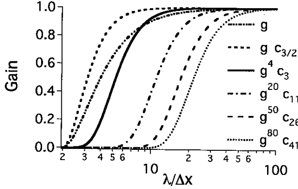
Figure 4: Gain versus wavelength for the bilinear filter without compensation ( g = g(1/2, k) ), with compensation ( g \cdot c_{3/2} = g(1/2, k) \cdot g(3/2, k) ), and n -pass bilinear filters with compensation ( g^n \cdot c_{\alpha_c} = g(1/2, k)^n \cdot g(\alpha_c, k) ) for n = 4, 20, 50 and 80 .
