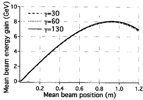
Figure 19: Average beam energy gain versus longitudinal position (in the laboratory frame) from 2D-1/2 simulations of a full scale 10GeV LPA in a boosted frame at \gamma = 30, 60 and 130, using the Yee solver.
