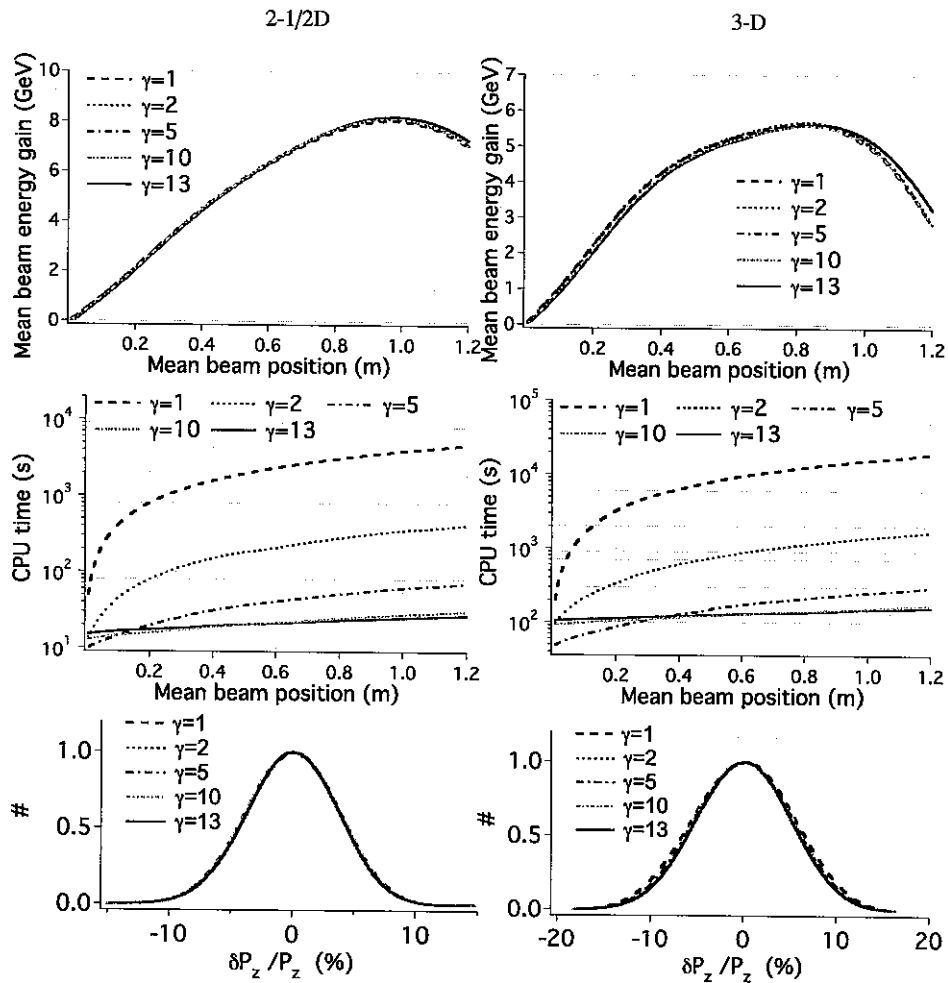
Figure 13: (top) Average scaled beam energy gain and (middle) CPU time, versus longitudinal position in the laboratory frame from simulations; (bottom) distribution of relative longitudinal momentum dispersion at peak energy, in the laboratory frame ( \gamma = 1 ) and boosted frames at \gamma = 2, 5, 10 and 13.
