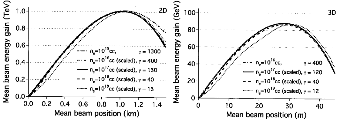
Figure 30: Average beam energy gain versus longitudinal position (in the laboratory frame) for simulations at n_e = 10^{19} cc down to 10^{15} cc, using frames of reference between \gamma = 12 and \gamma = 1300 , in 2-1/2D (left) and 3D (right).
