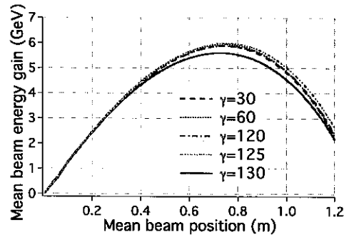
Figure 22: Average beam energy gain versus longitudinal position (in the laboratory frame) from 3D simulations of a full scale 10GeV LPA in a boosted frame at \gamma = 30, 60, 120, 125 and 130 , using the Yee solver ( \gamma = 30 and 60 ) and the CK2 solver ( \gamma = 120 - 130 ), with digital filter S(1) and with the time step set by c\delta t/\delta z = 1/\sqrt{2} for stability (see discussion below).
