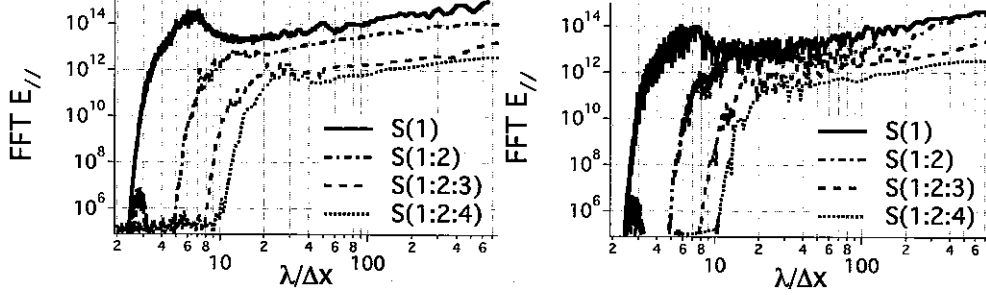
Figure 23: Fourier Transform of the longitudinal electric field at t=40 ps, averaged over plane on axis perpendicular to laser polarization, from (left) 3D and (right) 2D-1/2 simulations of a full scale 10GeV LPA in a boosted frame at \gamma = 130 , using the Yee solver and various smoothing kernels. The same time step at the 3D CFL limit c\delta t = \delta x / \sqrt{3} was used for both simulations.
