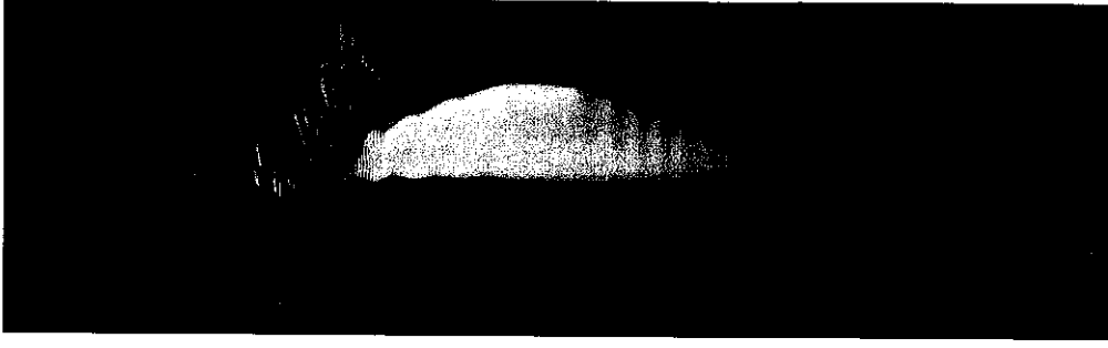
Figure 3: Snapshot of a surface plot of the longitudinal field from a 2-1/2D simulation of a full scale 10GeV LPA in a boosted frame at \gamma = 130 (elevation is proportional to the magnitude of the electric field). The laser is propagating from left to right and the plasma from right to left. A fast growing short wavelength instability is developing at the front of the plasma.
