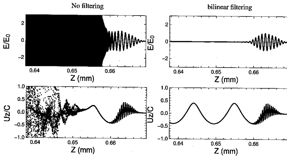
Figure 32: Snapshots from transverse electric field (normalized to maximum laser amplitude E_0 ) and plasma electrons longitudinal phase space projection, from a 1D simulation of a laser wakefield acceleration stage the CFL limits ( c\delta t = \delta x ) with (left) no filtering of current density; (right) application of a bilinear digital filter to the current density.
