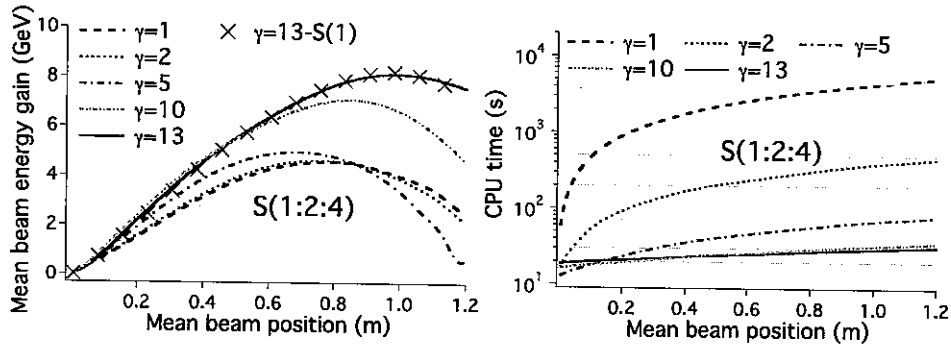
Figure 15: (left) Average scaled beam energy gain and (right) CPU time, versus longitudinal position in the laboratory frame from simulations in the laboratory frame ( \gamma = 1 ) and boosted frames at \gamma = 2, 5, 10 and 13 , using the Yee solver with digital filter S(1:2:4) (grey cross is reference from run with filter S(1)).
