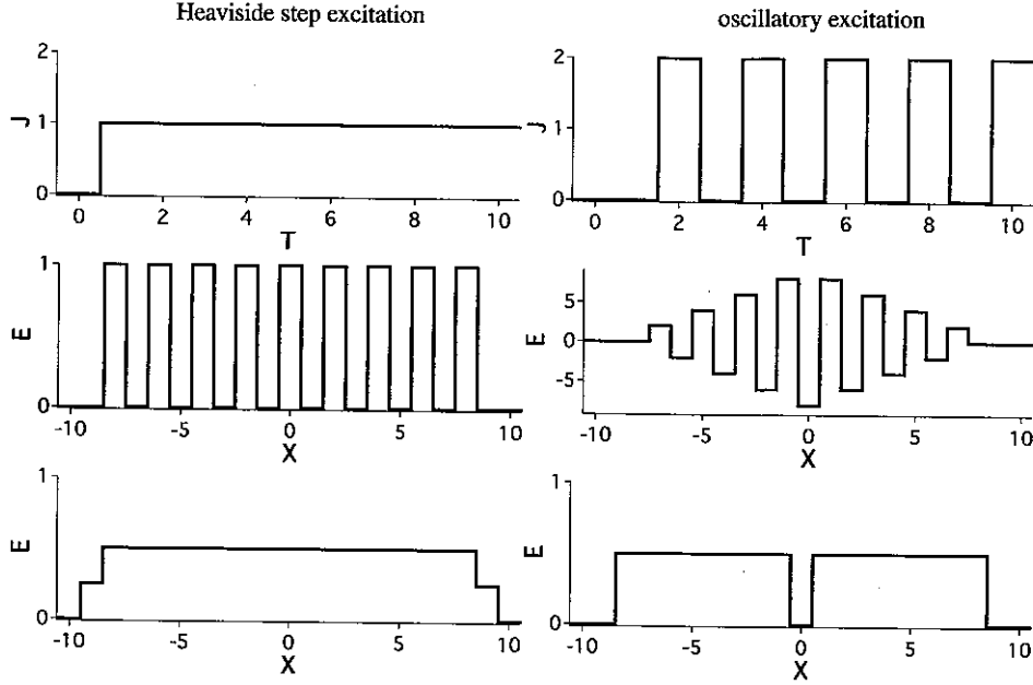
Figure 31: (top) time history (in time steps) of the current source for (left) a Heaviside step (right) a heaviside step modulated by a sinusoidal oscillation at the Nyquist frequency; (middle) response of the system of equations (73)-(74) via a snapshot of the electric field after 10 time steps, without filtering of the source term; (bottom) response of the system of equations (73)-(74) with application of bilinear digital filter of the source term in space. A time step of c\delta t = \delta x was used in all runs and scaled constants c = \epsilon_0 = 1 were assumed.
