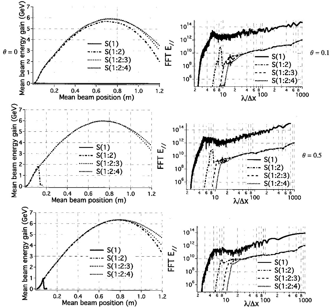
Figure 20: (left) Average beam energy gain versus longitudinal position (in the laboratory frame); (right) Fourier Transform of the longitudinal electric field at t=40 ps, averaged over plane on axis perpendicular to laser polarization, from 3D simulations of a full scale 10GeV LPA in a boosted frame at \gamma = 130 , using the Cole-Karkkainen-Friedman solver and various smoothing kernels, with (top) no numerical damping ( \theta = 0 ), (middle) damping with \theta = 0.1 and (bottom) \theta = 0.5 .
