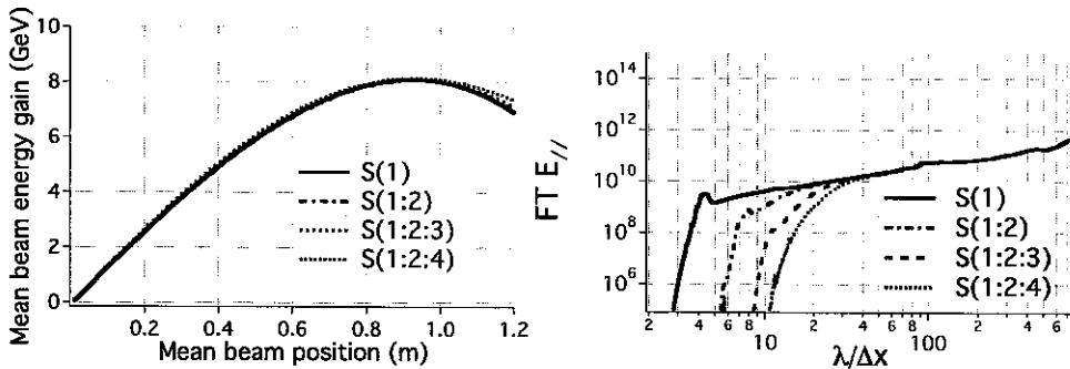
Figure 18: (left) Average beam energy gain versus longitudinal position (in the laboratory frame), (right) Fourier Transform of the longitudinal electric field at t=40 ps, averaged over whole domain, from 2D-1/2 simulations of a full scale 10GeV LPA in a boosted frame at \gamma = 130 , using the Yee solver and various digital filter kernels. Square cells ( \delta x = \delta z = 6.5 \mu\text{m} ) and the CFL time step ( c\delta t/\delta z = 1/\sqrt{2} ) were used.
