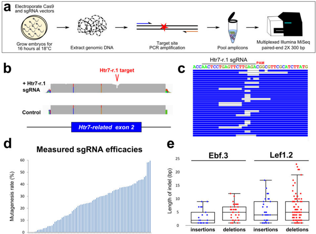
Figure 1. Next-Generation Sequencing approach to validating sgRNAs for use in Ciona embryos a) Schematic for next-generation sequencing approach to measuring mutagenesis efficacies of sgRNAs expressed in F0 Ciona embryos. See results and materials and methods for details. b) Representative view in IGV browser of coverage (grey areas) of sequencing reads aligned to the reference genome. “Dip” in coverage of reads from embryos co-electroporated with Eef1a1 > Cas9 and U6 > Htr7-r. 1 sgRNA vector indicates CRISPR/Cas9-induced indels around the sgRNA target site, in the 2 nd exon of the Htr7-related ( Htr7-r ) gene. Colored bars in coverage indicate single-nucleotide polymorphisms/mismatches relative to reference genome. c) Diagram representing a stack of reads bearing indels of various types and sizes, aligned to exact target sequence of Htr7-r. 1 sgRNA. d) Plot of mutagenesis efficacy rates measured for all sgRNAs, ordered from lowest (0%) to highest (59.63%). Each bar represents a single sgRNA. e) Box-and-whisker plots showing the size distribution of insertions and deletions caused by Ebf.3 or Lef1.2 sgRNAs.
