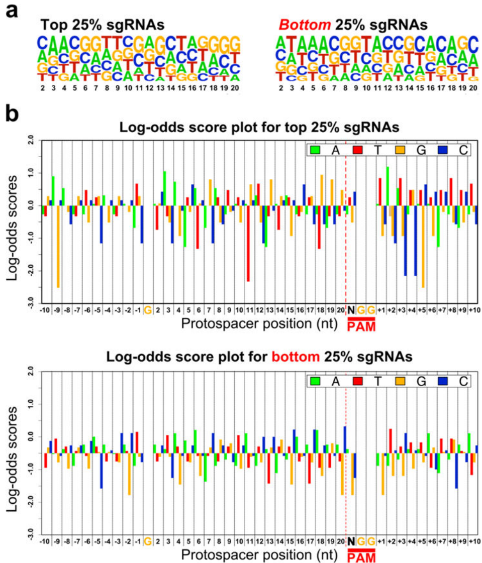
Figure 2. Correlations between sgRNA sequence composition and mutagenesis efficacy a) WebLogos representing the nucleotide composition at each variable position of the protospacer (nt 2–20, X axis), in top 25% and bottom 25% performing sgRNAs. b) Log-odds scores depicting the frequency of occurrence for nucleotides in the top 25% and bottom 25% sgRNAs, at all positions of the protospacer, PAM, and flanking regions. Position “1” of the protospacer has been omitted from the analysis, due to this always being “G” for PolIII-dependent transcription of U6-promoter-based vectors. Likewise, the “GG” of the PAM has also been omitted, as this sequence is invariant in all targeted sites. Positive and negative log-odds scores reflect abundance and depletion, respectively, of a specific nucleotide at a given position relative to its random occurrence in our sample space. See materials and methods for details.
