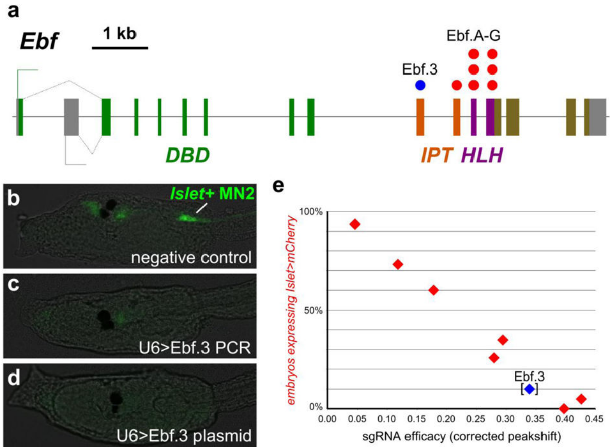
Figure 6. Linear relationship between sgRNA efficacy and mutant phenotype frequency in F0 a ) Diagram of Ebf locus, showing exons coding for DNA-binding (DBD), IPT, and helix-loop-helix (HLH) domains. Colored dots indicate exons targeted by the Ebf -targeting sgRNAs used to validate the OSO-PCR method for genetic loss-of-function. b ) Larvae co-electroporated with Sox1/2/3>nls::Cas9::nls , Islet>eGFP , and 25 \mu l (~2.5 \mu g) unpurified U6>NegativeControl PCR or c ) 25 \mu l (~2.5 \mu g) unpurified U6>Ebf.3 PCR, or d ) 25 \mu g U6>Ebf.3 plasmid. Islet>eGFP reporter plasmid is normally expressed in MN2 motor neurons (“ Islet + MN2”, green), which is dependent on Ebf function. Islet>eGFP was expressed in MN2s in 75 of 100 negative control embryos. In embryos electroporated with unpurified U6>Ebf.3 PCR products or U6>Ebf.3 plasmid, only 16 of 100 and 17 of 100 embryos, respectively, had Islet>eGFP expression in MN2s. This indicates similar loss of Ebf function in vivo by either unpurified PCR or purified plasmid sgRNA delivery method. c ) Plot comparing mutagenesis efficacies of the OSO-PCR-generated sgRNAs indicated in panel (a) (measured by Sanger sequencing, see text for details) and the ability to cause the Ebf loss-of-function phenotype (loss of Islet>mCherry reporter expression in MN2s in Sox1/2/3>H2B::eGFP+ embryos). The nearly perfect inverse correlation between sgRNA mutagenesis efficacy and Islet>mCherry expression indicates a linear relationship between sgRNA activity and mutant phenotype frequency in electroporated embryos. Ebf.3 sgRNA data point is bracketed, because its mutagenesis efficacy was not measured by Sanger sequencing but comes from the NGS data collected in this study.
