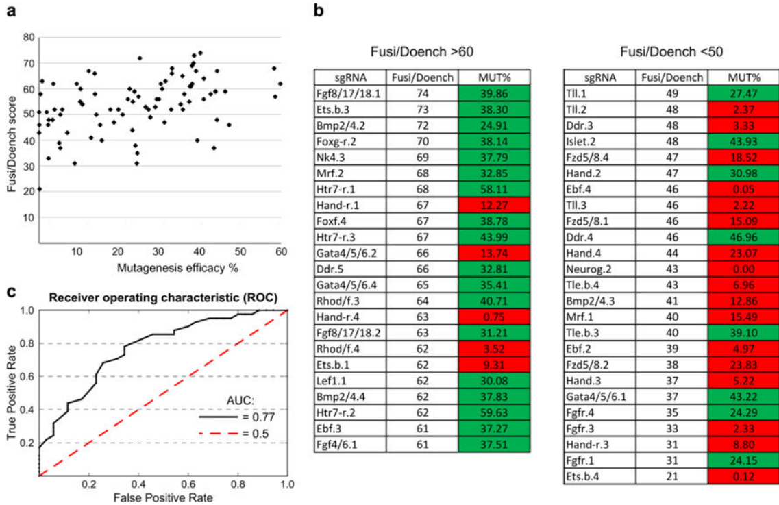
Figure 3. Using Fusi/Doench scores to predict mutagenesis efficacies of sgRNAs in Ciona a) Mutagenesis efficacy rate of each sgRNA plotted against the same sgRNA's Fusi/Doench algorithm score, obtained from CRISPOR. The Spearman's rank correlation coefficient ( \rho ) is 0.435 ( p = 3.884e-05 ). b) sgRNAs grouped by sorted Fusi/Doench predicted scores (left: >60; right: <50). 18 of 23 sgRNAs of Fusi/Doench score over 60 showed a measured mutagenesis efficacy (MUT%) over 24%, classified as "good" (shaded green). In contrast, only 4 from the same set had a MUT% under 24%, classified as "bad". "Good" and "bad" classifications were based on phenotype frequency in F0 (see text for details). Out of 25 sgRNAs with Fusi/Doench score under 50, 17 were "bad", while only 8 were "good". c) A Receiver Operating Characteristic (ROC) curve assesses the credibility of using Fusi/Doench score cutoff (from 0 to 100) to classify sgRNAs as either "good" (>24.5% efficacy) or "bad" (< 24.5% efficacy). Using Fusi/Doench cutoffs as such a classifier returns an AUC of 0.77 (black line), while an AUC of 0.5 (dashed red line) represents the performance of a classifier solely based on random chance. The optimal Fusi/Doench cutoff (above which a score is likely to indicate "good" sgRNAs) was found to be between 50 and 55. See materials and methods and Supplementary Table 2 for details.
