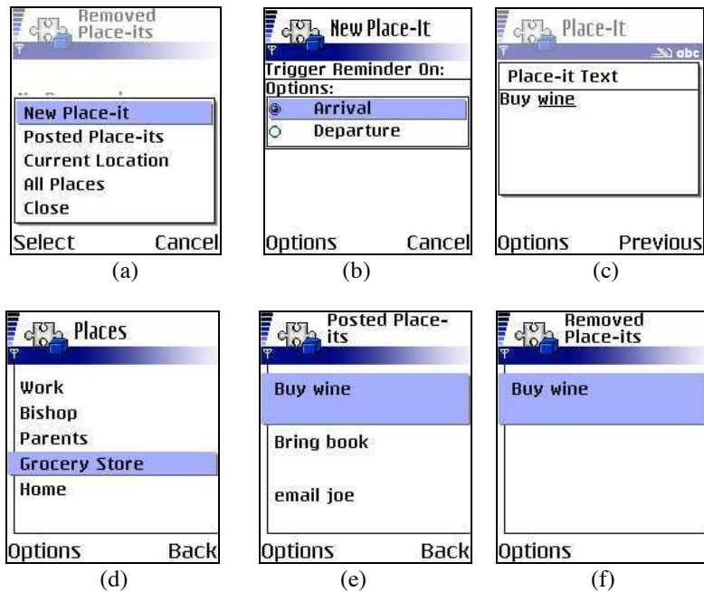
Figure 1. (a) Creating a new Place-It note; (b) Setting the note to be triggered upon arrival; (c) Typing the text of the note; (d) Posting the note to the 'Grocery Store'; (e) Showing all posted Place-It notes; (f) The reminder is triggered when Jill arrives at the grocery store and the note is removed.
