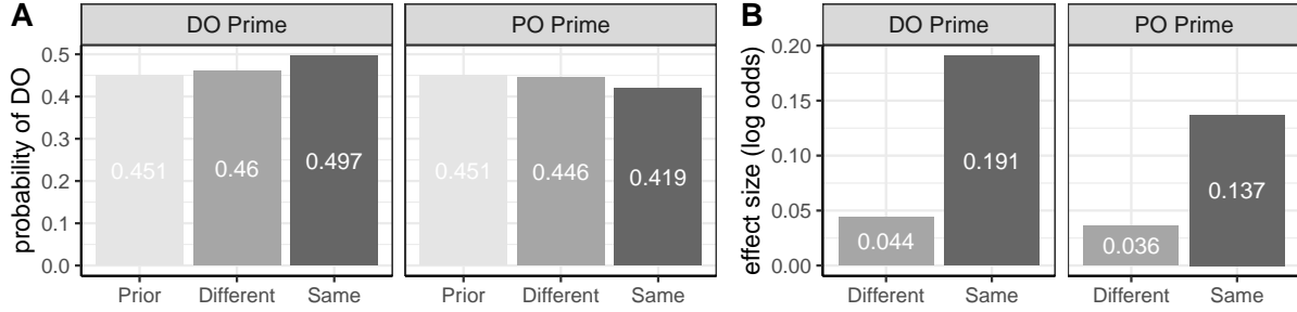
Figure 2: Results of Simulation 1. Panel A : Model-estimated average prior and posterior probability of DO for the target verbs in Pickering and Branigan (1998); Same refers to the condition with verb overlap between the prime and the target; Different refers to the condition without verb overlap. Panel B : Model-predicted priming effect size, calculated as the difference of log-odds between the posterior and the prior for DO.
