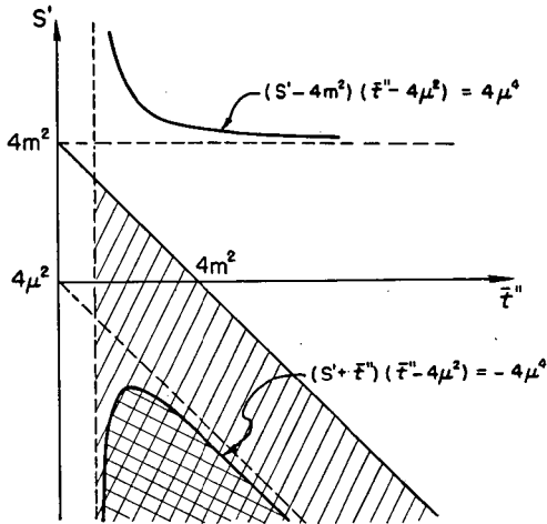
FIG. 2. The region of integration in Eq. (A.17) is shaded. The curve which encloses the double cross-hatched region is the boundary where the Legendre expansion fails. It has its maximum at s' = -8\mu^2 , t'' = 6\mu^2 .
