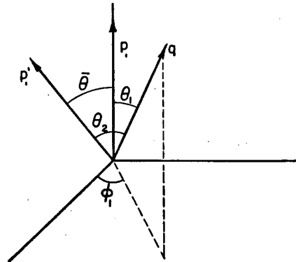
FIG. 3. Coordinate system for evaluation of the two-pion intermediate state contribution to the negative cut.
