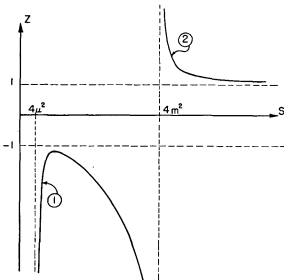
FIG. 1. Curves showing the domain of validity of the Legendre polynomial expansion of the nucleon-antinucleon amplitude. The allowed region is that above curve 1 and below curve 2. Outside this region the expansion definitely diverges.
