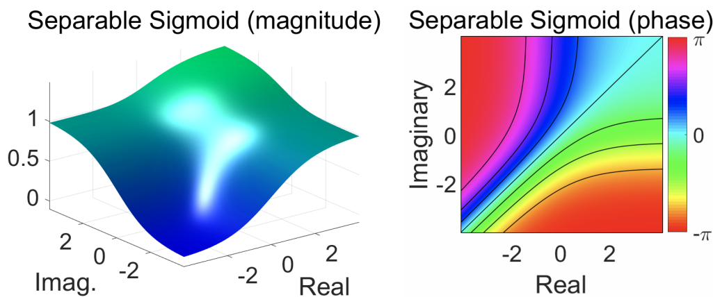
Figure 2.11: Magnitude (left) and phase (right) output of the separable sigmoid activation function applied to the complex plane.
