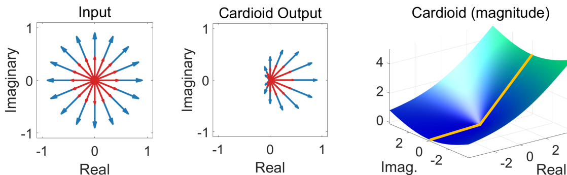
Figure 2.17: Our new cardioid activation function is a phase-sensitive complex extension of ReLU. Left / Center: Each arrow indicates a sample input/output of our cardioid function on the complex plane. Right: The magnitude transformation of the cardioid function shows that it is reduced to ReLU on the real axis (orange line).
