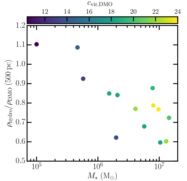
Figure 8. The correlation between M_* and the central density reduction in the hydrodynamic runs relative to the DMO runs at 500 pc. There is little to no reduction in central density below 10^6 M_{\odot} , while more massive systems see significant reduction. This figure offers a complementary view of Figure 7, in which density reduction is shown as a function of radius scaled by r_{1/2} : it shows the density reduction at a fixed physical radius. The coloring of the points indicates the concentration of each galaxy’s halo in the DMO run.
