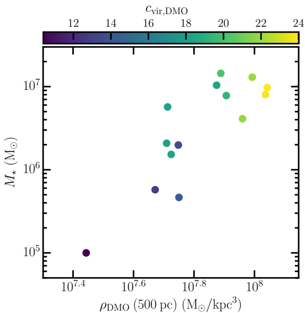
Figure 10. Relationship between stellar mass and central dark matter density in the DMO runs. There is a clear correlation between the stellar mass formed and the amplitude of the density profile at 500 pc in the DMO version of each simulation; this figure is equivalent to taking a slice through the left panel of Figure 9 at 500 pc. The coloring of each point shows the measured concentration in the DMO run.
