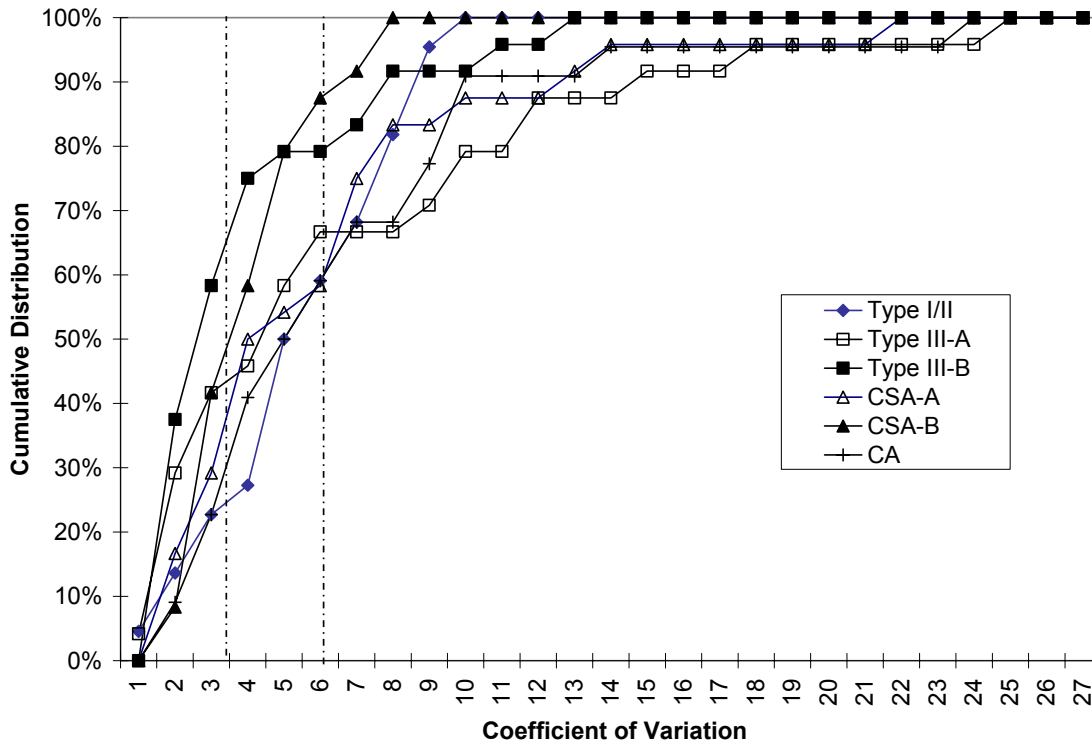
Figure 3.18. Flexural strength test variability by cement type.
