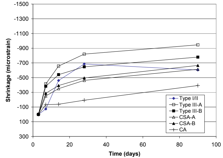
Figure 4.14d. 40°C + ~0% RH (Dry and Hot).
