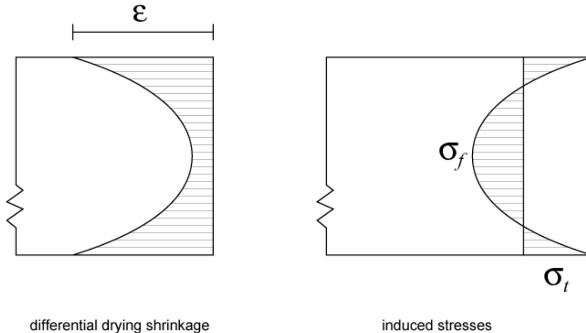
Figure 3.13. Self-balanced stress on the beam cross section caused by drying shrinkage gradient.
