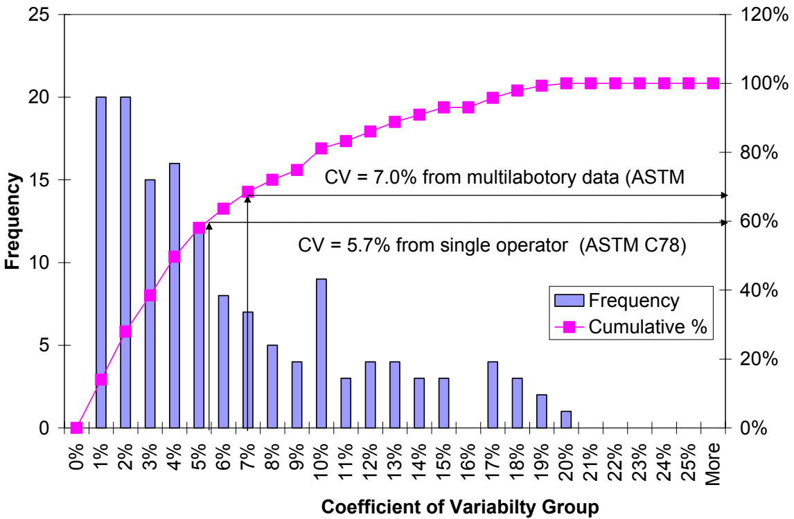
Figure 3.14b. Flexural strength.
