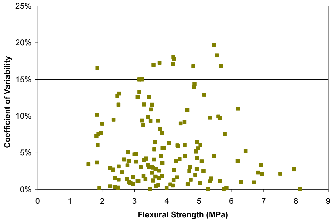
Figure 3.16b. Flexural strength.
