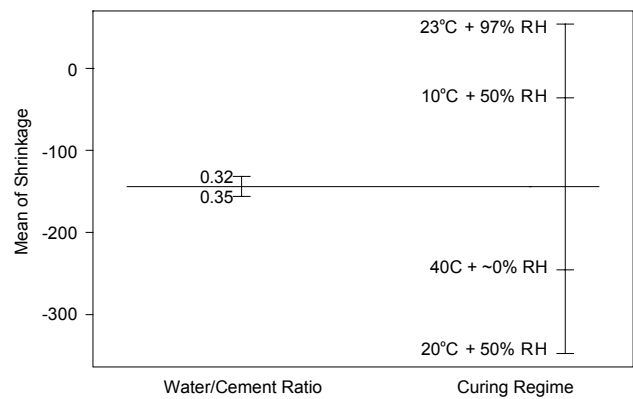
Figure 4.18f. Calcium Aluminate (CA).
