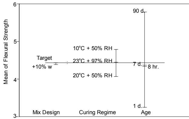
Figure 3.27c. Type III-B Portland cement.
