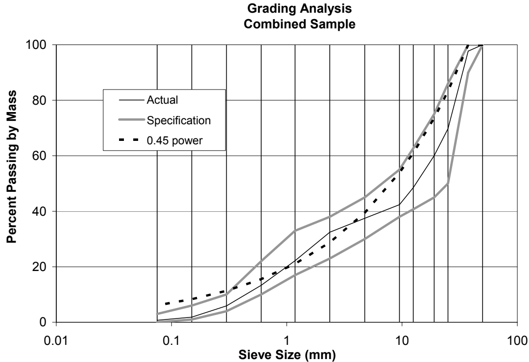
Figure 2.1. Grading analysis.
