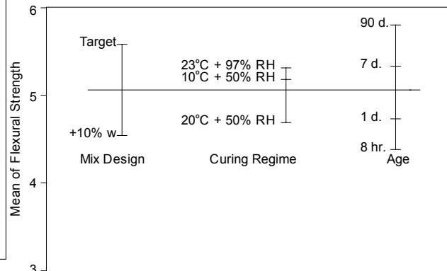
Figure 3.27f. Calcium Aluminate (CA).
