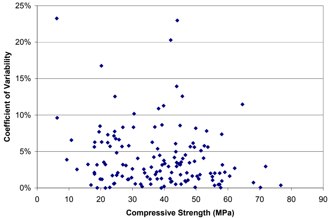
Figure 3.16a. Compressive strength.
