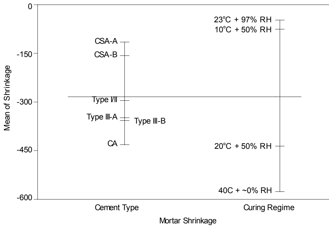
Figure 4.17b. Mortar specimens.
