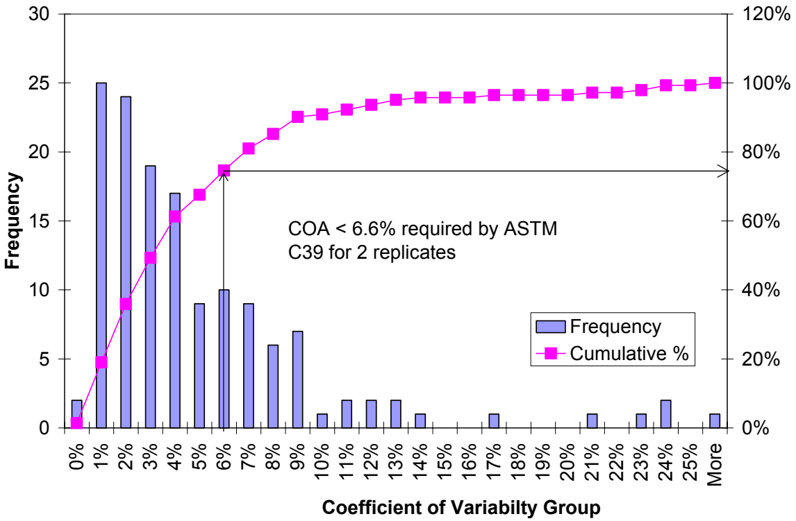
Figure 3.14a. Compressive strength.
