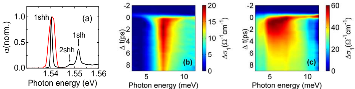
Fig. 1. (a) Near-infrared absorption spectrum of the GaAs multiple quantum wells at a temperature of T = 6 K (black curve). The red curve represents the spectrum of the near-infrared pump pulses. (b) and (c) photoinduced conductivity change \Delta\sigma_1 measured by THz spectroscopy as function of frequency and delay time \Delta t for and excitation density of n_0 \sim 10^{10} \text{ cm}^{-2} (b) and n \sim 5 n_0 (c).
