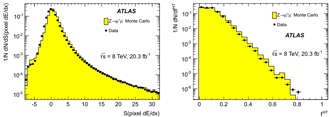
Fig. 2 Normalised distributions of the dE/dx significance in the pixel system, S(\text{pixel } dE/dx) , (left) and f^{\text{HT}} , the fraction of TRT hits passing the high threshold, (right) for muons from Z \rightarrow \mu\mu events in data and simulation
