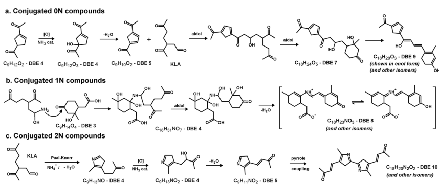
Scheme 2 Proposed formation of plausible highly-conjugated species in C_{500} that may contribute to the visible-light-absorbing properties of C_{500} . Likely, many isomers and higher-order oligomers exist. Molecular formulas shown in the scheme, with their proposed corresponding structures, have been detected with HR-MS (Table 1).
