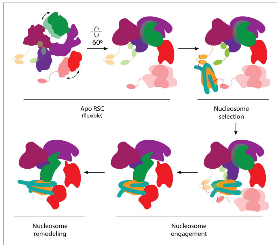
Figure 6. Proposed model of nucleosome engagement. Mechanistic model of RSC engaging a nucleosome. The apo RSC is shown with its moving tail and leg lobes, and its flexibly attached histone-tail binding domains. The BrDs bind and select target nucleosomes with acetylated tails. The selected nucleosome engages RSC, first through the arm lobe of the core, which then positions the ATPase domain at the end of the leg to be able to bind SHL2. During nucleosome remodeling, the ATPase translocates the DNA while the RSC core holds onto the histone core.
