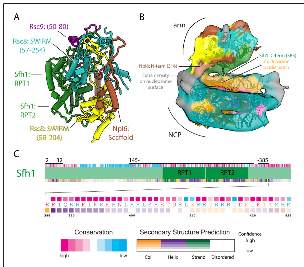
Figure 4. Architecture of the arm lobe and its interaction with the NCP. (A) The structure of the RSC arm lobe with protein domains and segments labeled. (B) The density of the NCP and arm region from the RSC-NCP reconstruction showing the connections that occur between the two. (C) Domain organization, sequence conservation and secondary structure prediction for Sfh1. Below is a zoomed in view of the C-terminus showing the sequence at a residue level. The domain map coloring is the same as in (Figure 1—figure supplement 4).
