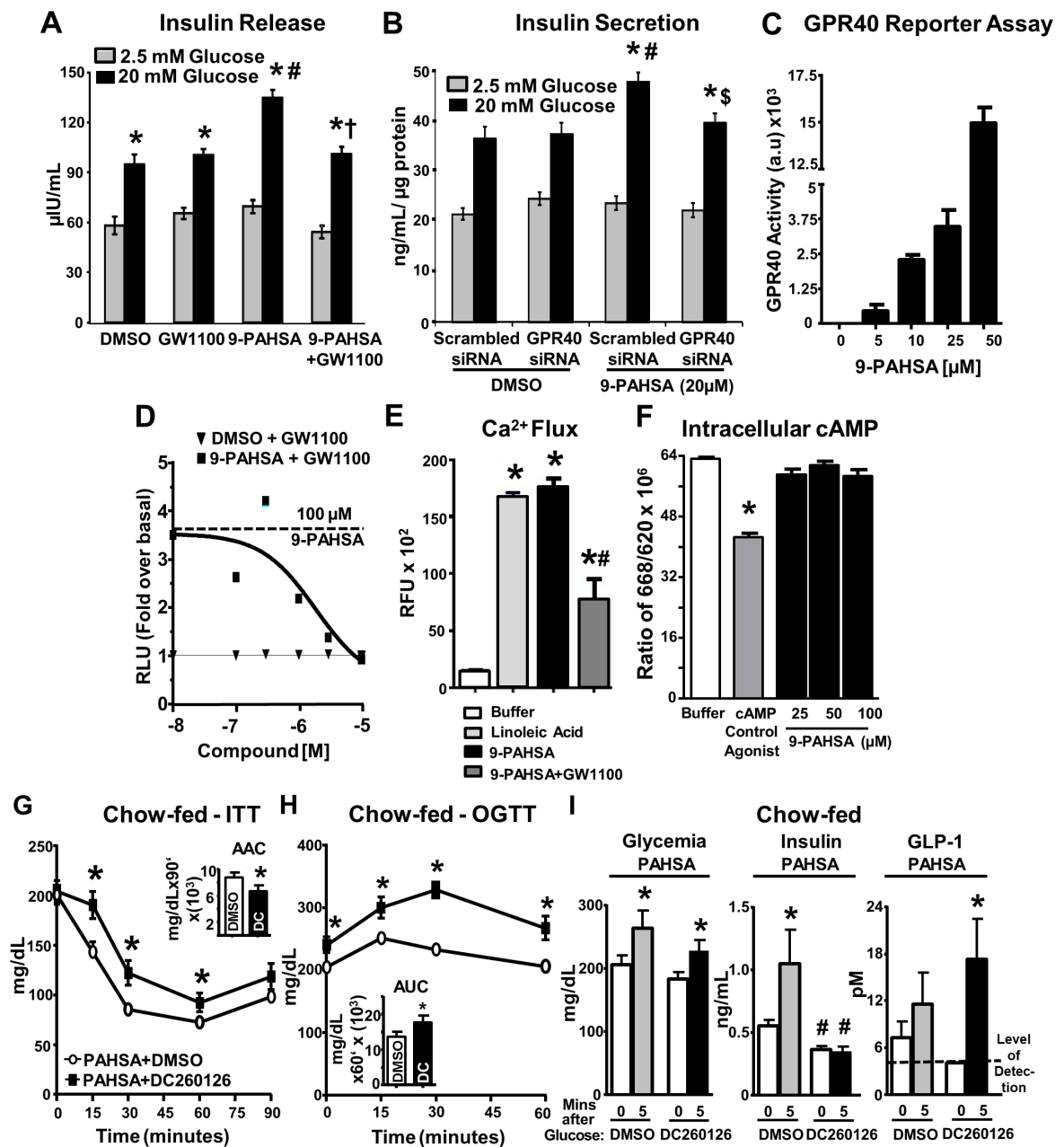
Figure 2. PAHSAs directly activate GPR40, and GPR40 antagonism reverses PAHSA-mediated improvements in glucose tolerance, insulin sensitivity and insulin secretion
