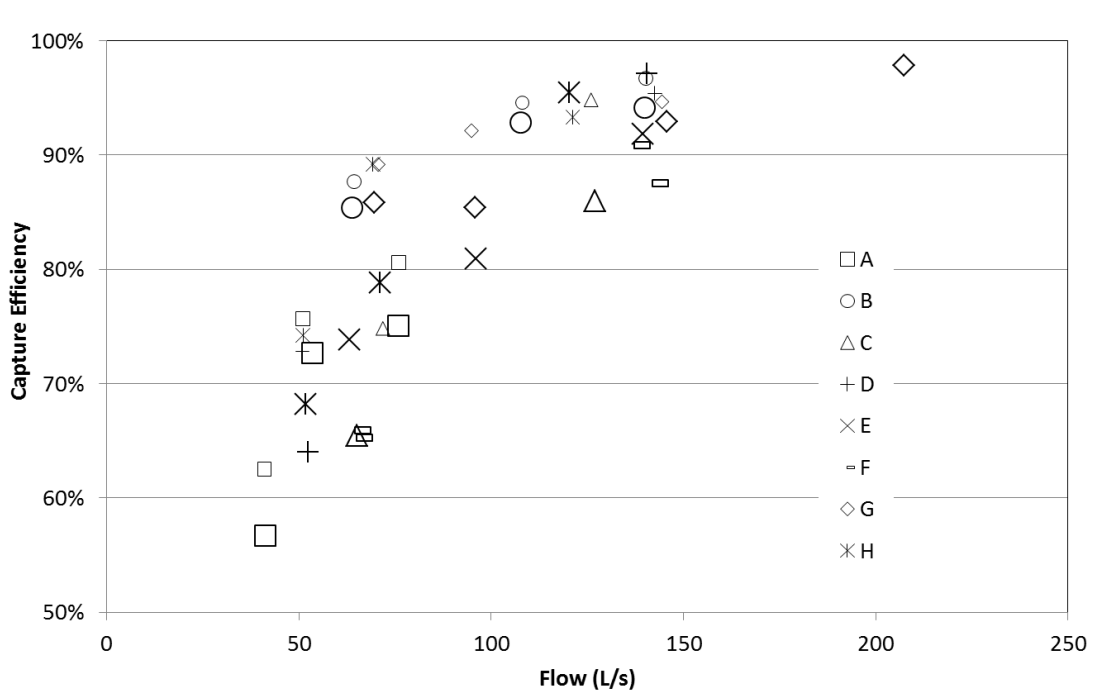
Figure 8. Capture efficiency versus airflow for the eight range hood models tested for the initial test method (larger symbols for the higher mounting level and the smaller symbols for the lower mounting level)
