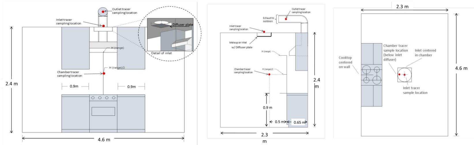
Figure 3. Schematic of the capture efficiency test chamber
